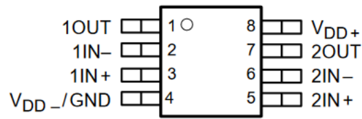
Figure 3-2. TLV2432x: PW Package, 8 Pin TSSOP (Top View)
