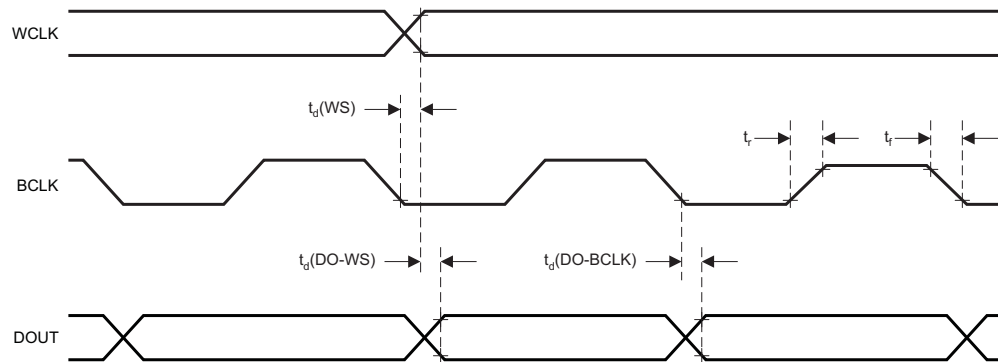
Figure 1. I²S/LJF/RJF Timing in Master Mode
