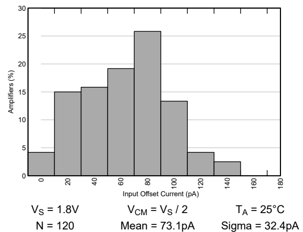
Figure 5-10. Input Offset Current Distribution
