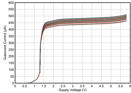
Figure 5-32. Quiescent Current vs Supply Voltage
