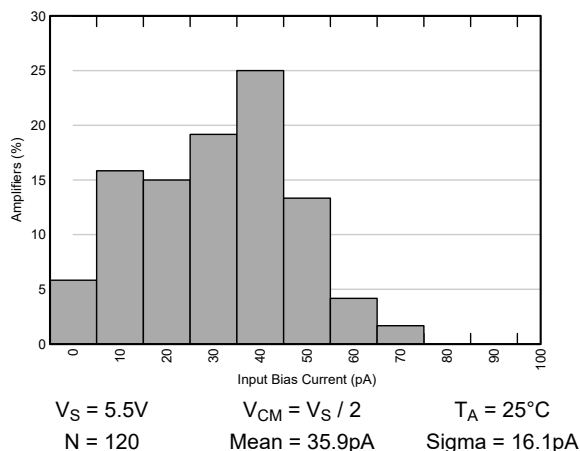
Figure 5-5. Input Bias Current Distribution
