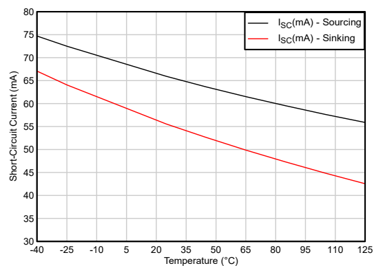
Figure 5-46. Short-Circuit Current vs Temperature
