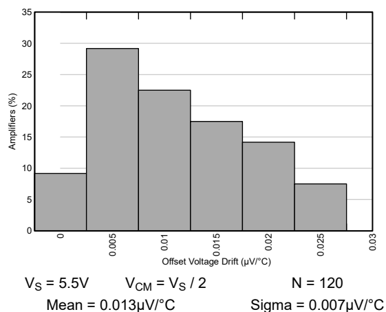
Figure 5-4. Offset Voltage Drift
