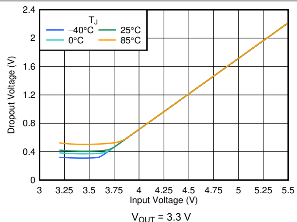
Figure 5-6. Dropout Voltage vs V_{IN}
