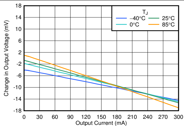
Figure 5-2. Load Regulation vs I_{OUT}
