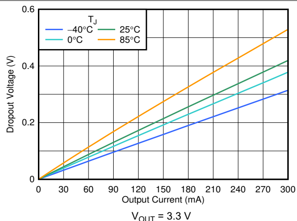
Figure 5-4. Dropout Voltage vs I_{OUT}
