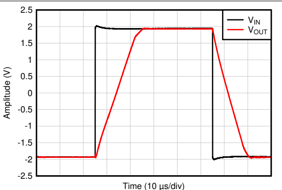
Figure 7-33. Overload Recovery
