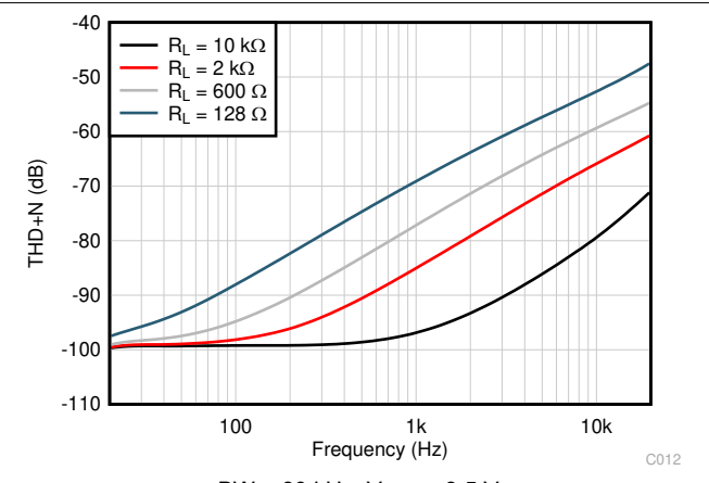
Figure 6-20. THD+N Ratio vs Frequency BW = 80 kHz, V_{OUT} = 3.5\text{ V}_{RMS}
