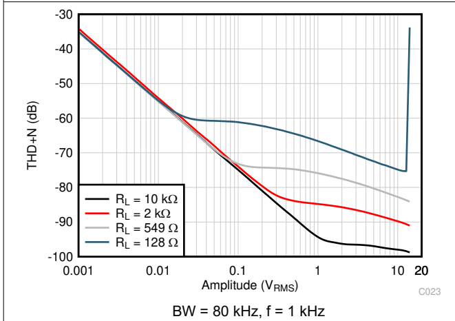
Figure 6-21. THD+N vs Output Amplitude BW = 80 kHz, f = 1\text{ kHz}
