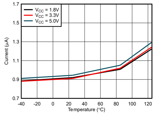
Figure 6-6. 10Hz I_{CAVG} vs Temperature
