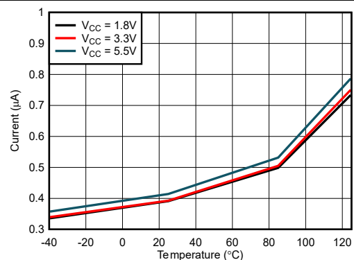
Figure 6-4. 1.25Hz I_{CAVG} vs Temperature
