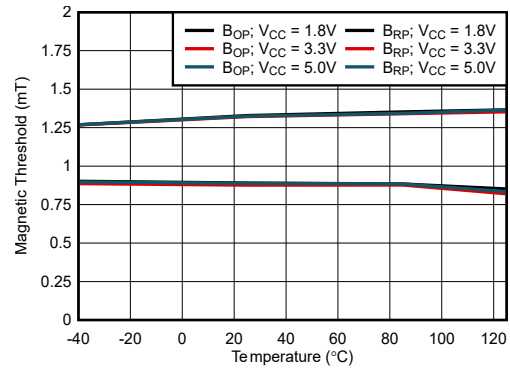
Figure 6-2. 1.3mT B_{OP} and B_{RP} Thresholds vs Temperature
