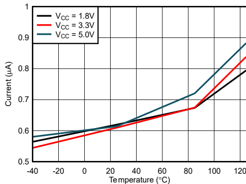
Figure 6-5. 5Hz I_{CAVG} vs Temperature
