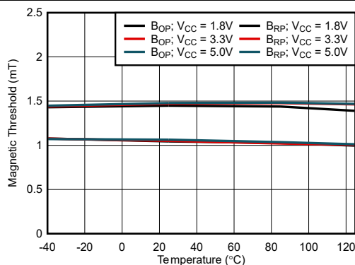
Figure 6-3. 1.5mT B_{OP} and B_{RP} Thresholds vs Temperature
