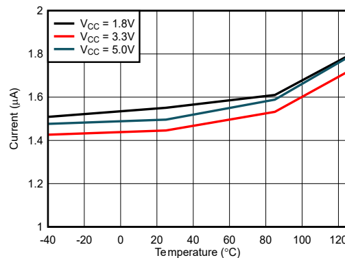
Figure 6-7. 20Hz I_{CAVG} vs Temperature
