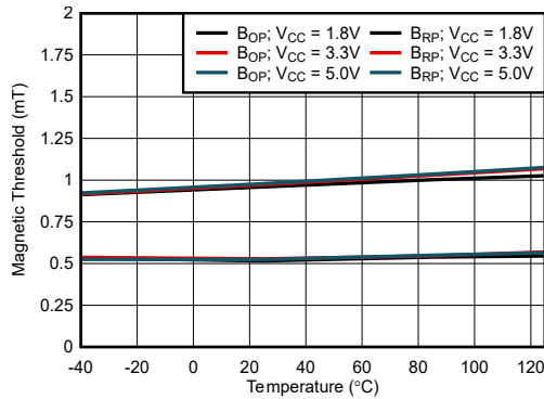
Figure 6-1. 1.0mT B_{OP} and B_{RP} Thresholds vs Temperature
