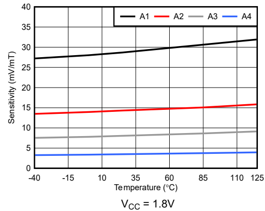
Figure 6-8. TMAG5253BA Sensitivity vs Temperature
