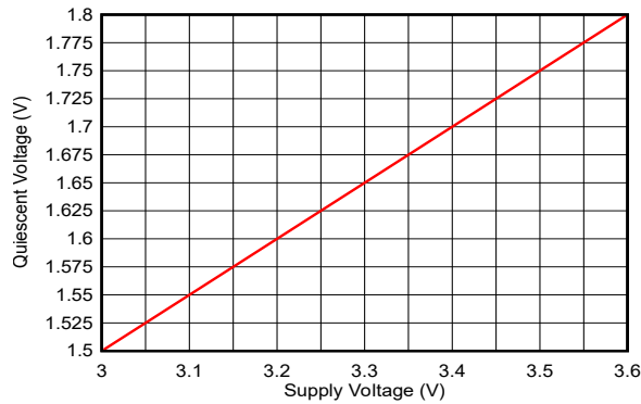
Figure 6-7. TMAG5253BA Quiescent Voltage vs Supply Voltage
