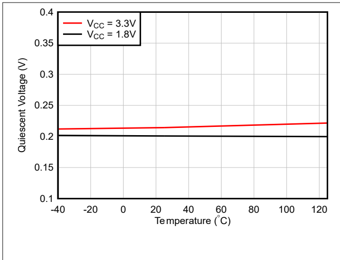
Figure 6-19. TMAG5253UA Quiescent Voltage vs Temperature
