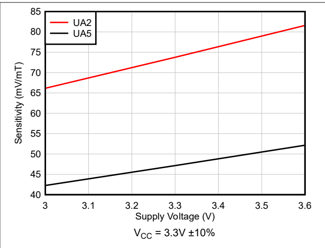
Figure 6-20. Sensitivity vs Supply Voltage
