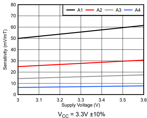
Figure 6-11. TMAG5253BA Sensitivity vs Supply Voltage
