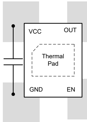
Figure 9-12. Layout Example
