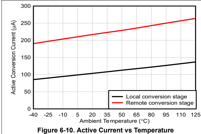
Figure 6-10. Active Current vs Temperature
