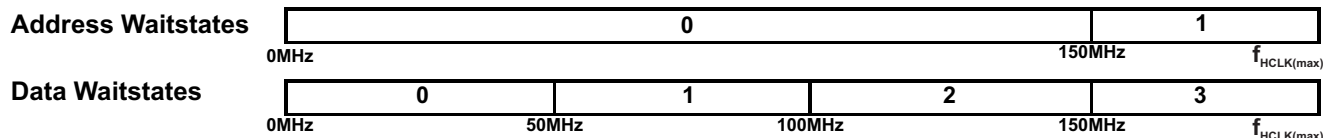
Figure 5-2. Wait States Scheme
