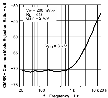
Figure 25. Common-mode Rejection Ratio vs Frequency
