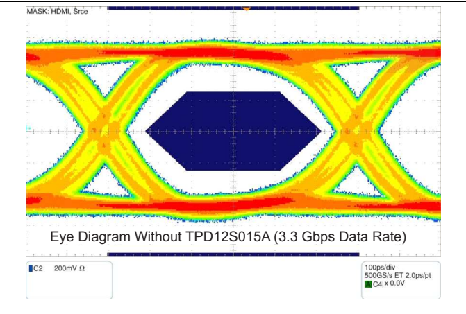
Figure 12. Eye Diagram Performance on a Test Board for the D+, D- Lines at 3.3 Gbps
