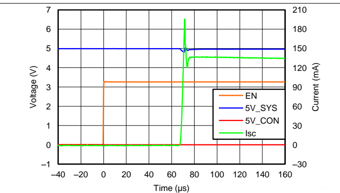
Figure 2. Enable to Short Circuit
