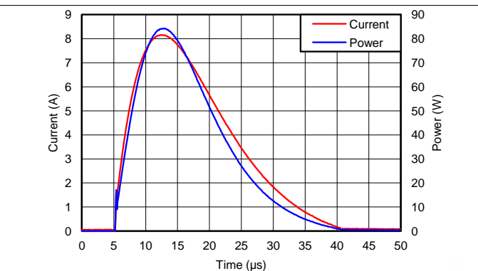
Figure 4. Utility Pin Surge Curves
