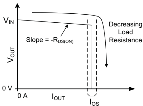
Figure 6. Output Characteristic Showing Current Limit
