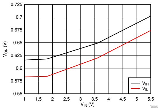
-40°C to +105°C Figure 7-5. ON Pin Threshold
