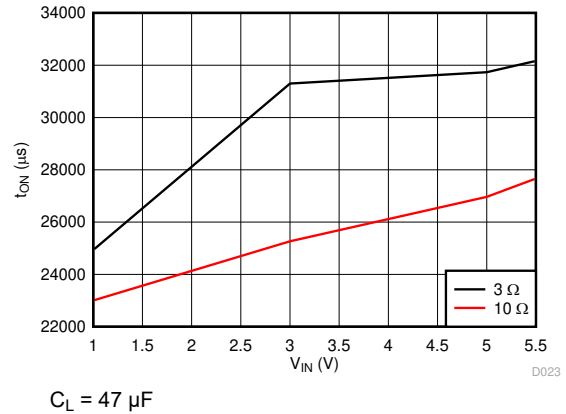
Figure 7-20. Turn-On vs Load Resistance (CT = 10000 pF)
