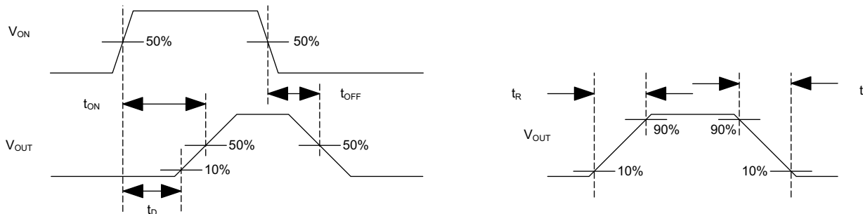
Figure 22. Timing Waveforms
