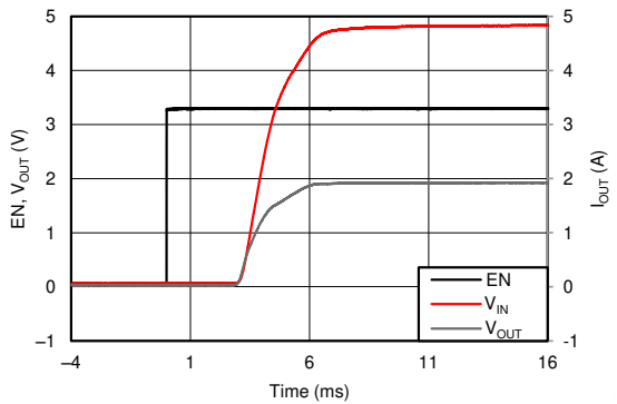
Figure 8-10. Turnon Delay and Rise Time 150 \mu\text{F} // 2.5 \Omega
