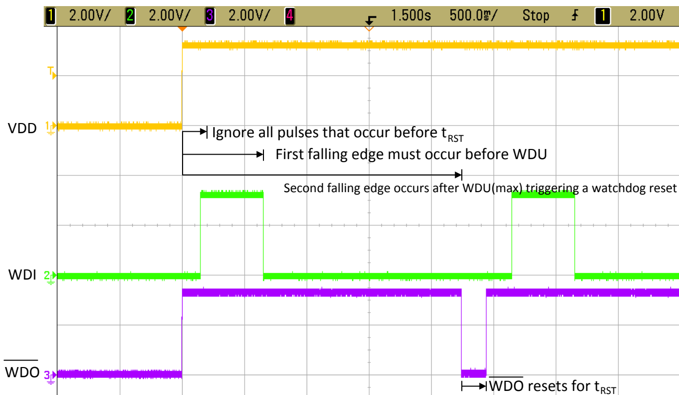
Figure 8-6. Watchdog Fault Caused by WDI Pulse Arriving Too Late (After t_{WDL(max)} )
