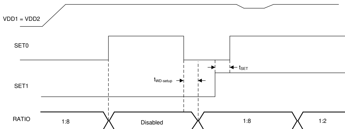
Figure 6-3. Changing SET0 and SET1 Pins
