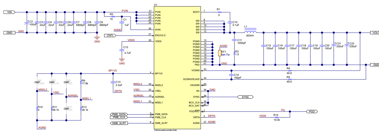
Figure 7-1. TPS546B24S Application
