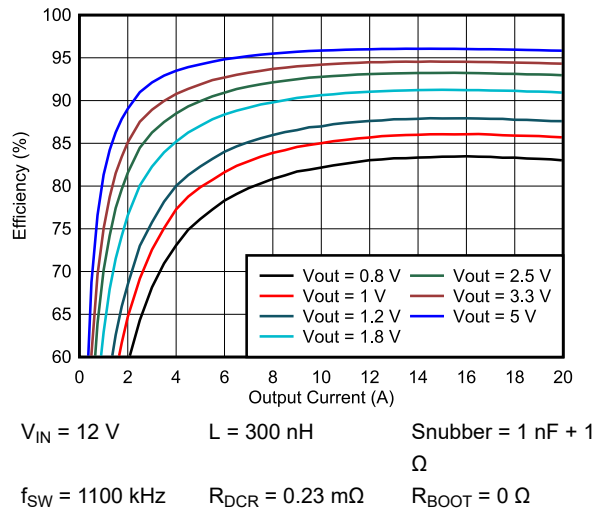
Figure 5-5. TPS546B24S Efficiency vs Output Current
