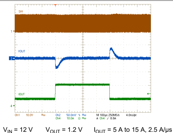
Figure 7-7. Load Transient Response
