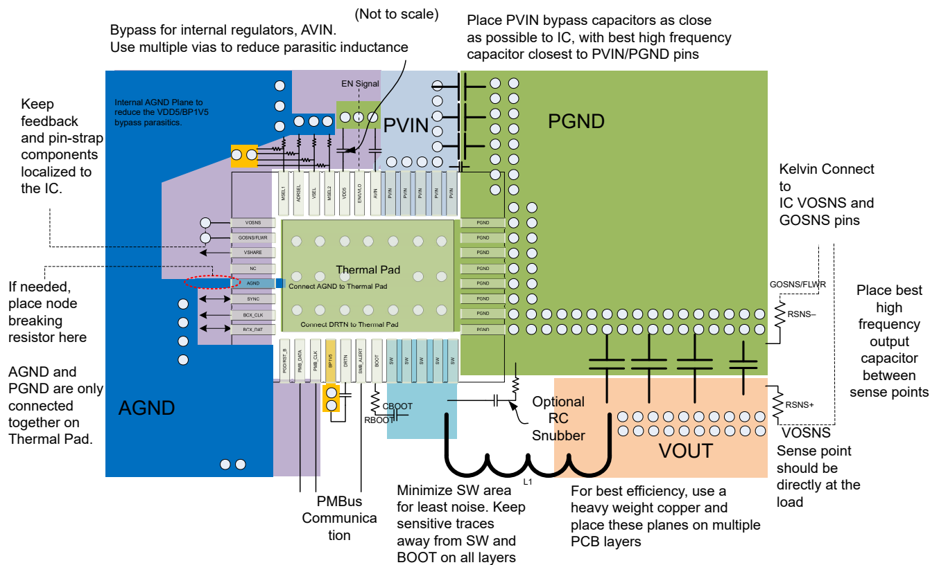
Figure 7-9. PCB Layout Recommendation
