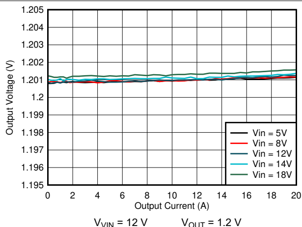
Figure 7-3. Load Regulation
