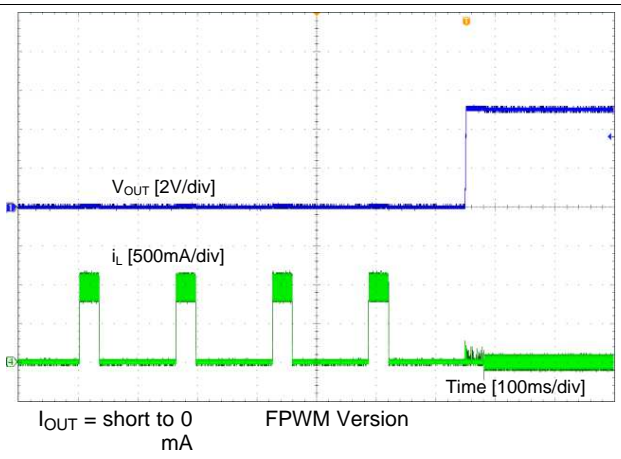
Figure 26. Short Recovery
