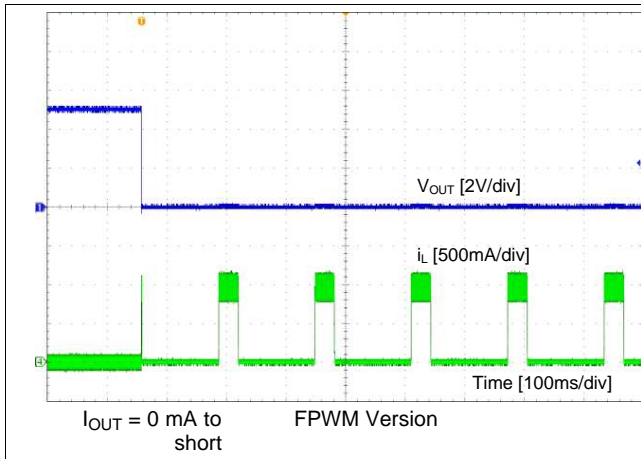
Figure 25. Short Protection
