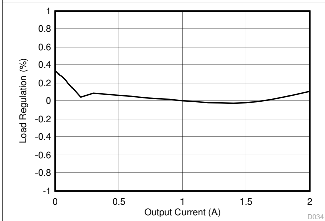
Figure 8-4. TPS562200 Load Regulation, V_I = 5V
