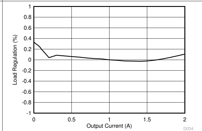
Figure 8-5. TPS562200 Load Regulation, V_I = 12V
