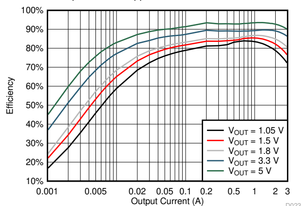
TPS563201 Efficiency
