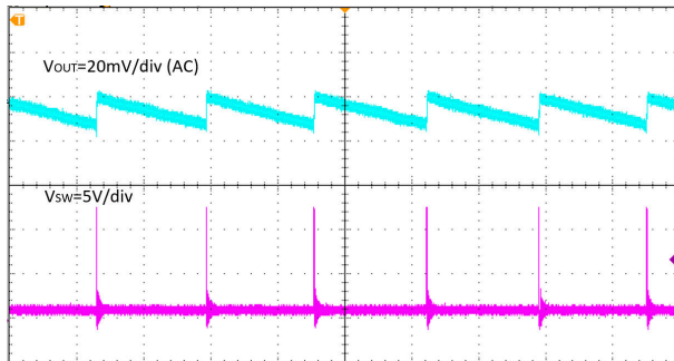
Figure 7-4. Output Voltage Ripple, I_{OUT} = 10\text{ mA} , Time = 80\ \mu\text{s/div}
