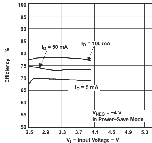
Figure 8-17. TPS65130 Efficiency vs Input Voltage
