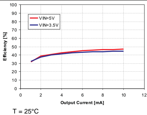
Figure 31. VEE Charge Pump Efficiency
