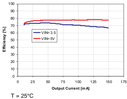
Figure 29. VN DCDC Efficiency
