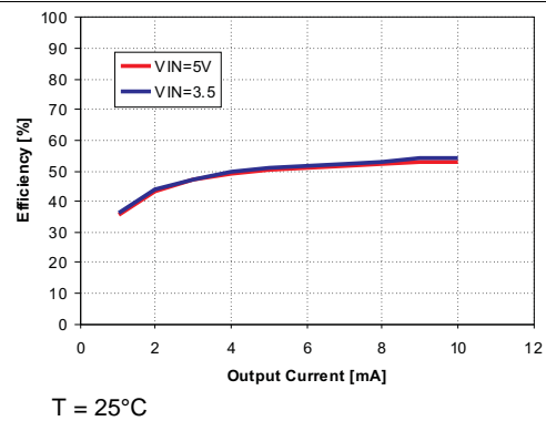
Figure 32. VDDH Charge Pump Efficiency
