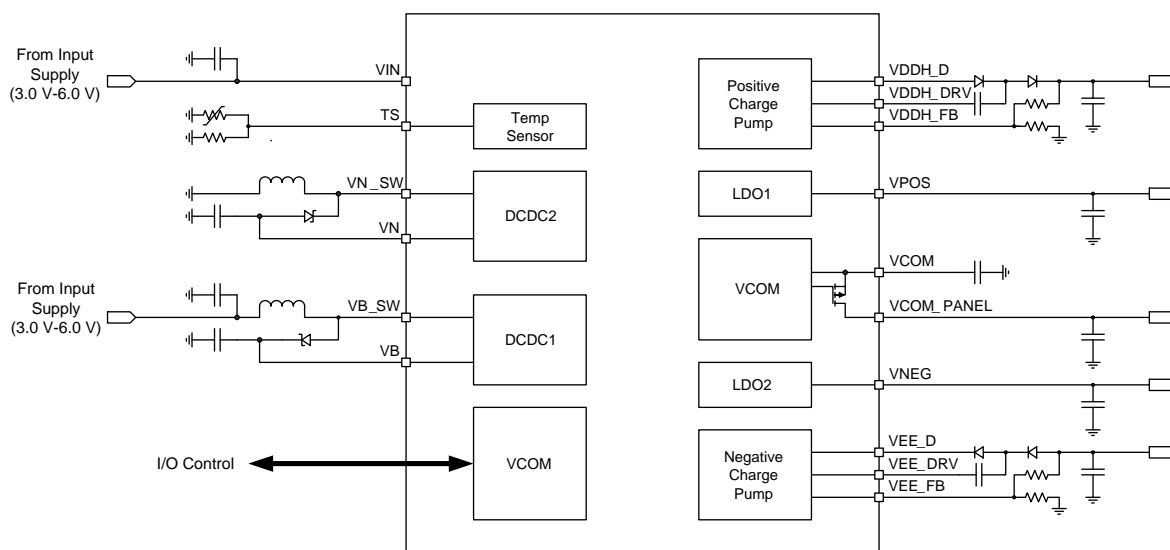
Typical Application Schematic
