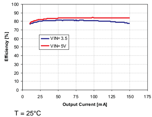
Figure 30. VB DCDC Efficiency
