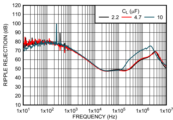
Figure 5-23. Ripple Rejection versus Output Capacitor ( C_L ) and Frequency (New Chip)
