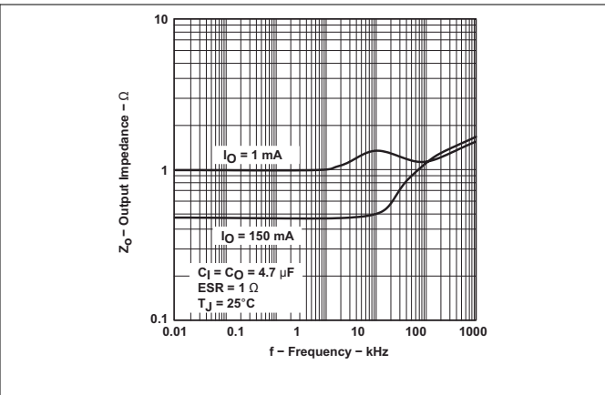
Figure 5-14. Output Impedance vs Frequency (Legacy Chip)
