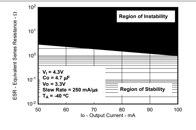
Figure 5-63. Typical Region of Stability ESR vs Output Current (Legacy Chip)
