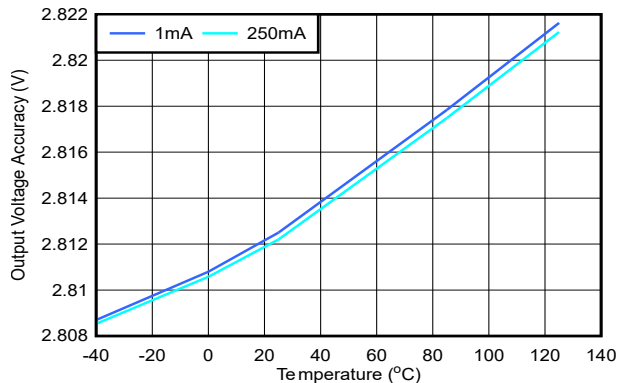
Figure 6-4. TPS794 Output Voltage vs Junction Temperature
