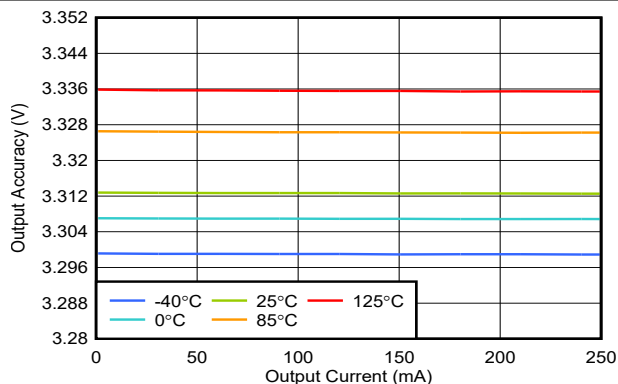
Figure 6-2. TPS794 Output Voltage vs Output Current
