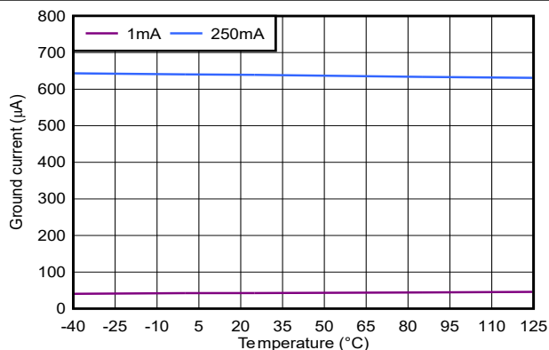
Figure 6-6. TPS794 Ground Current vs Junction Temperature
