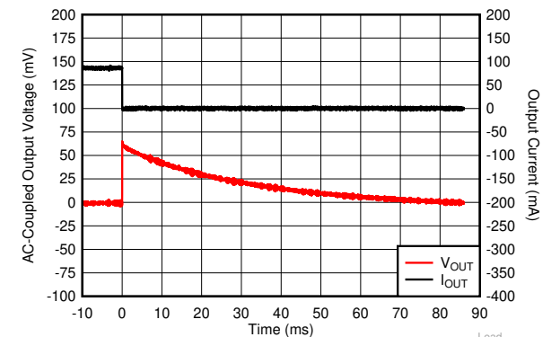
Figure 6-18. I_{OUT} Transient From 100 mA to 0 mA
