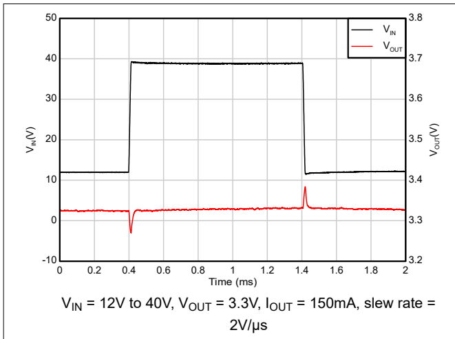
Figure 7-6. Line Transient
