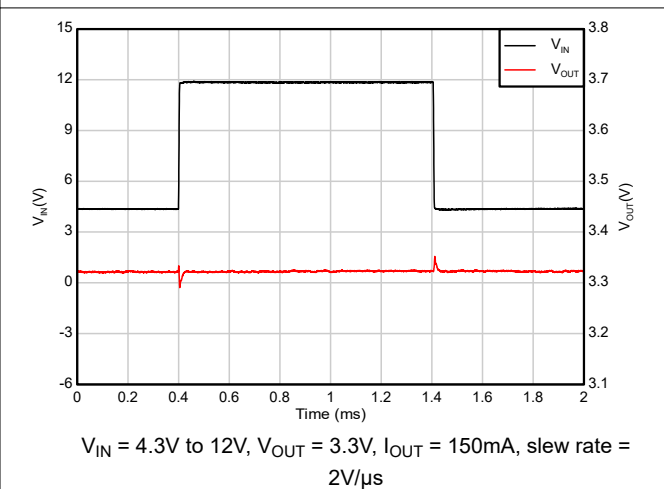
Figure 5-30. Line Transient
