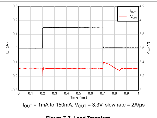
Figure 7-7. Load Transient
