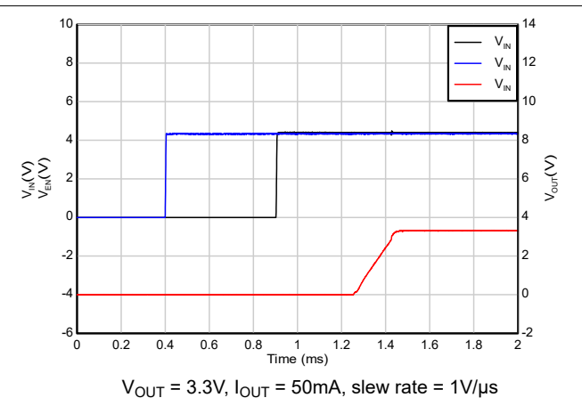
Figure 7-9. Start-up with Sequencing (IN after EN)
