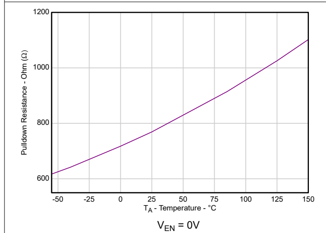
Figure 5-27. Output Discharge Resistance vs Temperature
