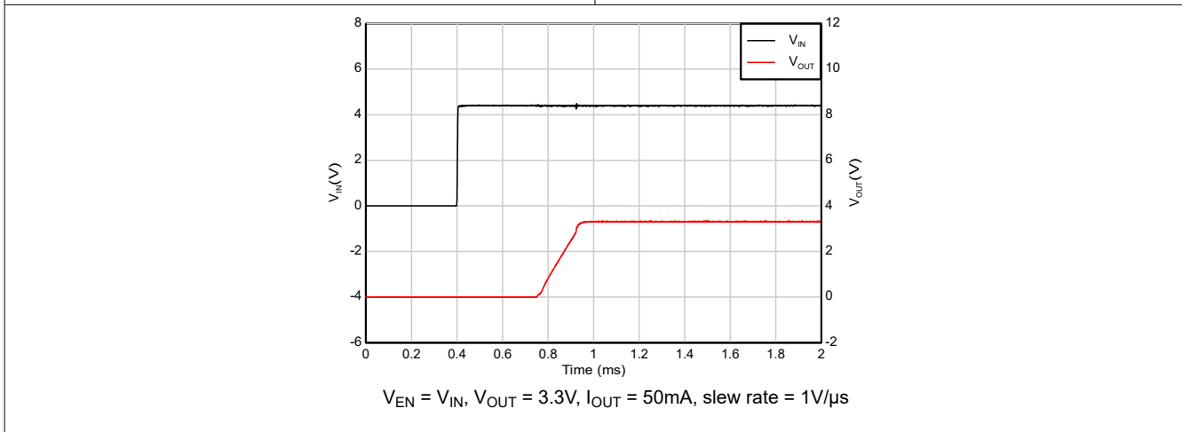
Figure 7-10. Start-up with IN and EN Tied Together
