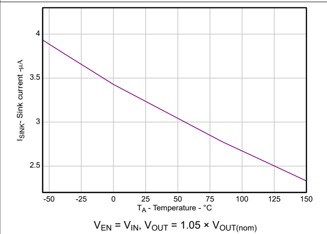
Figure 5-28. Output Sink Current vs Temperature
