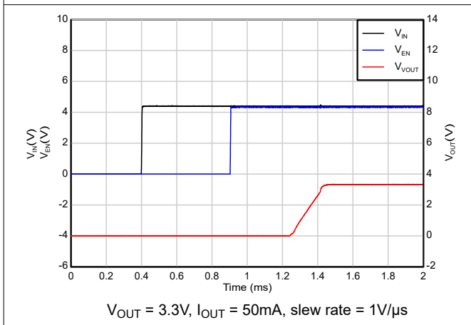
Figure 7-8. Start-up with Sequencing (EN after IN)
