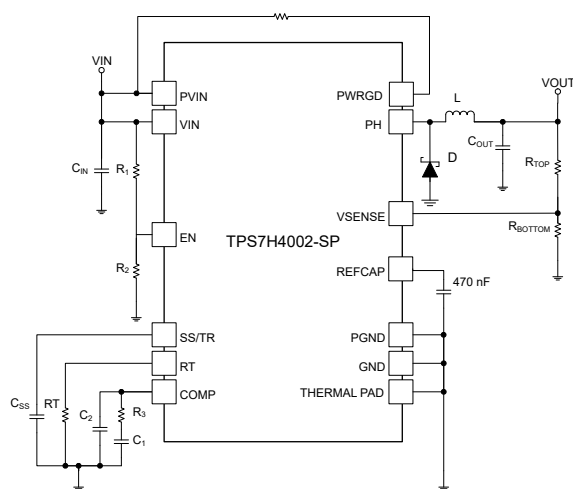
Functional Diagram
