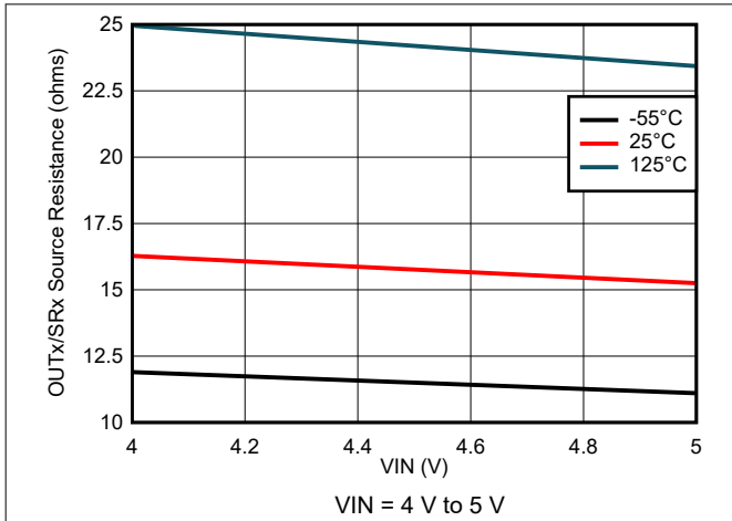
Figure 7-61. Output Source Resistance Variation
