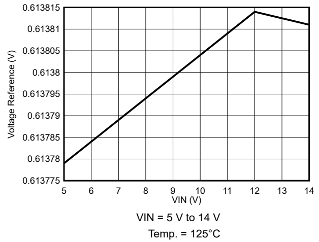
Figure 7-16. Voltage Reference Variation
