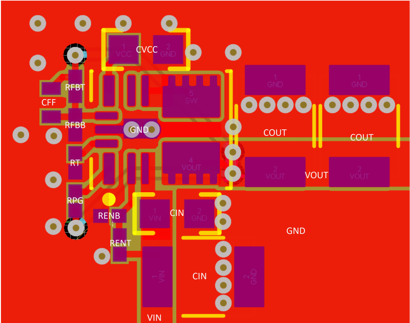
Figure 8-15. Example Layout
