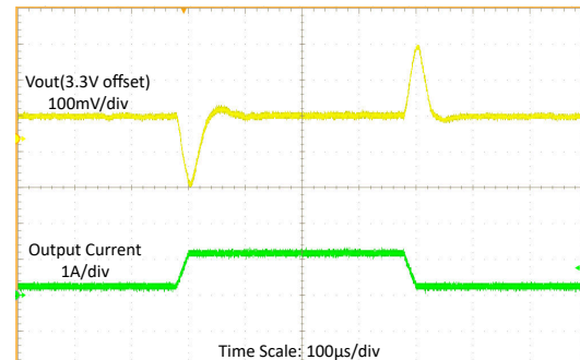
V_{IN} = 2.7V, V_{OUT} = 3.3V \quad I_{OUT} = 100mA \text{ to } 1A \text{ with } 20\mu s \text{ slew rate}
