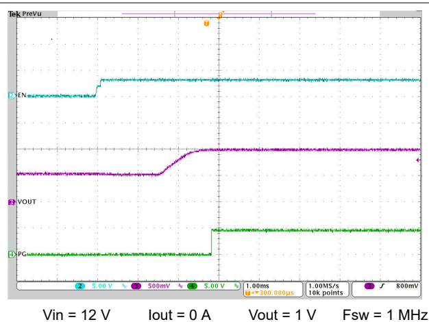
Figure 8-12. EN Start-up – 0.5-V Prebias
