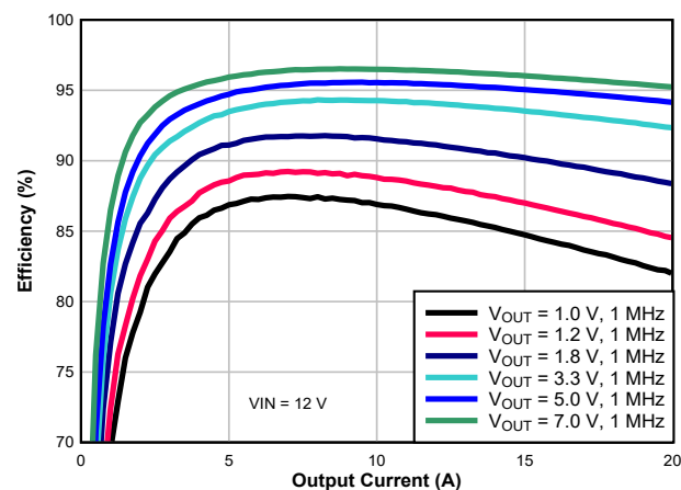
Typical Application Efficiency
