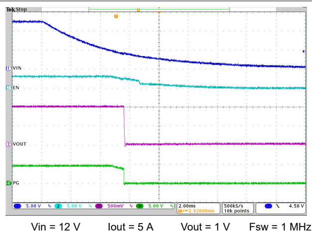
Figure 8-14. VIN Shutdown
