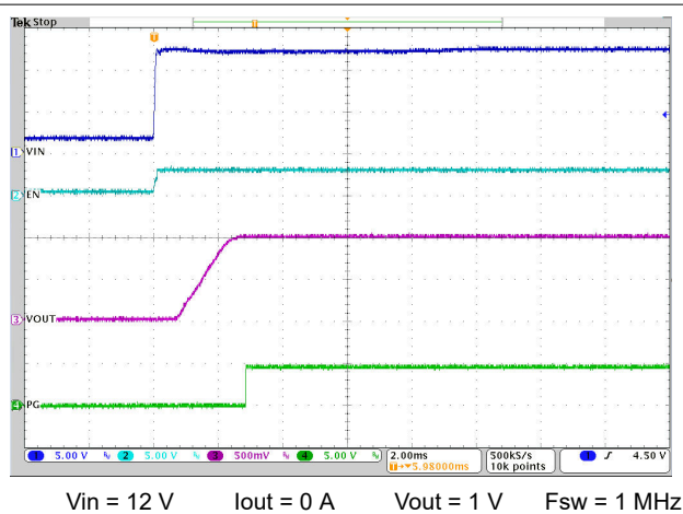
Figure 8-13. VIN Start-Up
