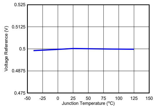
Figure 6-6. V REF
