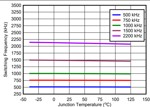
Figure 6-16. Switching Frequency vs Temperature
