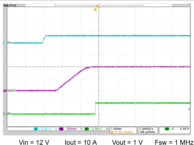
Figure 8-11. EN Start-up – With Load
