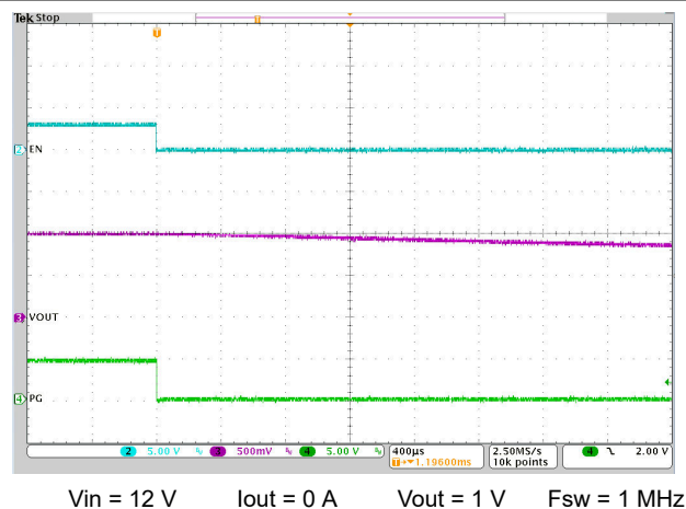
Figure 8-10. EN Shutdown
