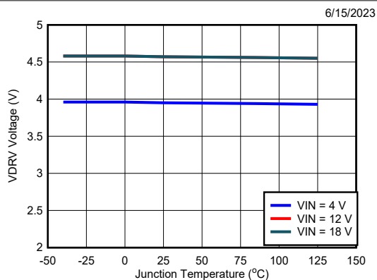
Figure 6-15. VDRV vs Temperature
