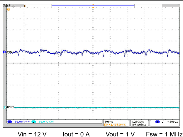
Figure 8-15. Input Ripple – No Load
