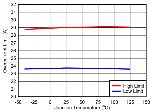
Figure 6-3. Overcurrent Limit
