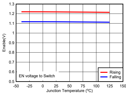
Figure 6-5. Enable Voltage
