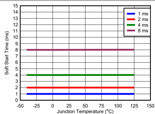
Figure 6-12. Soft Start
