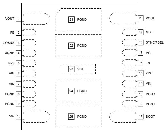
Figure 5-2. 25-Pin B3QFN-RDG Package (Top View)
