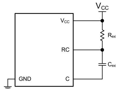
Figure 7-2. Timing Component Connection, Without External Ground
