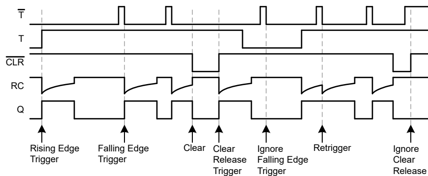
Figure 5-1. Timing Diagram
