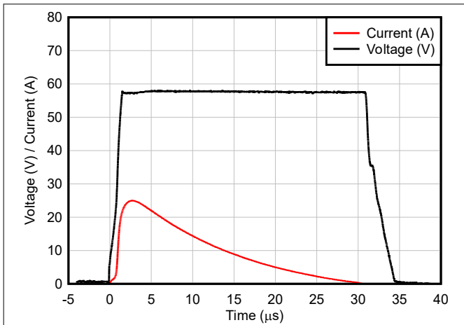
Figure 6-1. 8/20µs Surge Response at 25A
