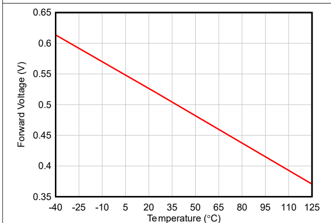
Figure 6-3. Forward Voltage vs Temperature
