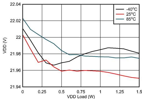
Figure 7-11. V_{VDD-VEE} Load Regulation: V_{IN} = 16.5\text{ V} , V_{VDD-VEE} = 22\text{ V} , V_{COM-VEE} = 4\text{ V}
