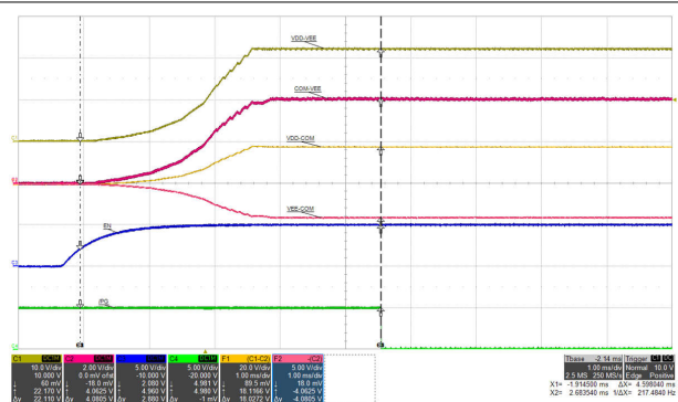
Figure 7-6. Start-up: V_{IN} = 15\text{ V} , V_{D\bar{D}-V\bar{E}E} = 22\text{ V} , V_{C\bar{O}M-V\bar{E}E} = 4\text{ V} , I_{V\bar{D}-V\bar{E}E} = 68\text{ mA} , No Load on V_{C\bar{O}M-V\bar{E}E} . Time Scale: 1ms/div.
