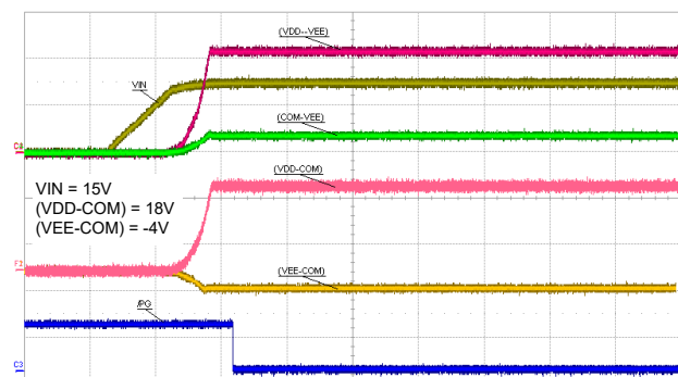
Typical Power-up Sequence
