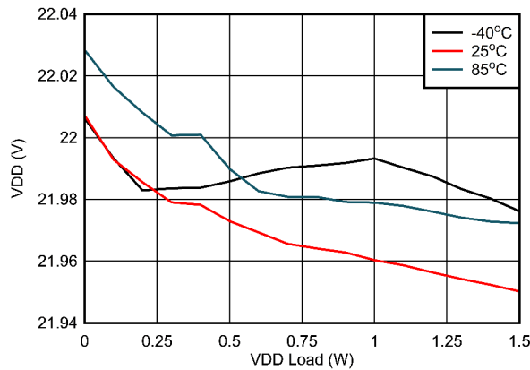
Figure 7-9. V_{VDD-VEE} Load Regulation: V_{IN} = 13.5\text{ V} , V_{VDD-VEE} = 22\text{ V} , V_{COM-VEE} = 4\text{ V}
