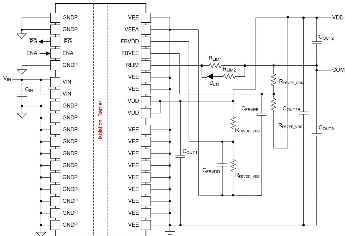
Figure 9-10. Dual output application schematic configured for \text{V}_{\text{COM\_VEE}} regulation < 2.5V
