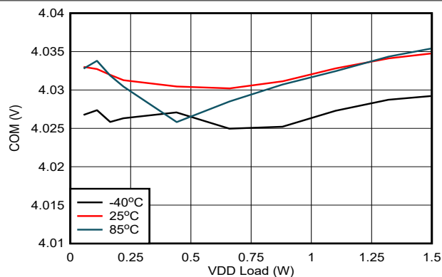
Figure 7-13. V_{COM-VEE} Load Regulation: V_{IN} = 15\text{ V} , V_{VDD-VEE} = 22\text{ V} , V_{COM-VEE} = 4\text{ V}
