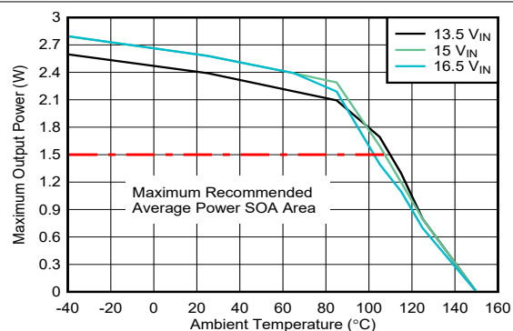
Figure 7-5. SOA Derating Curves: V_{D\bar{D}-V\bar{E}E} = 22\text{ V} , V_{C\bar{O}M-V\bar{E}E} = 4\text{ V} , T_{shut}=150^\circ\text{C} , No Load on V_{C\bar{O}M-V\bar{E}E} , tested in a shielded box.
