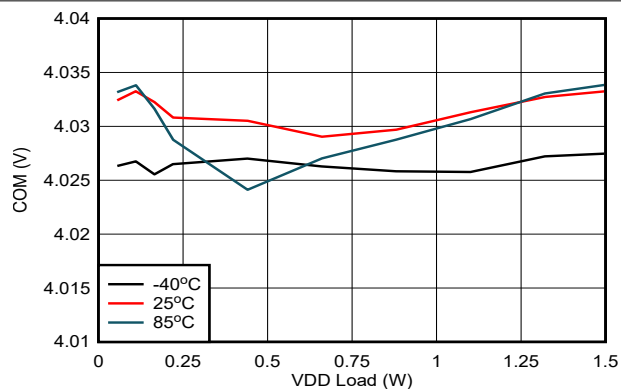
Figure 7-14. V_{COM-VEE} Load Regulation: V_{IN} = 16.5\text{ V} , V_{VDD-VEE} = 22\text{ V} , V_{COM-VEE} = 4\text{ V}
