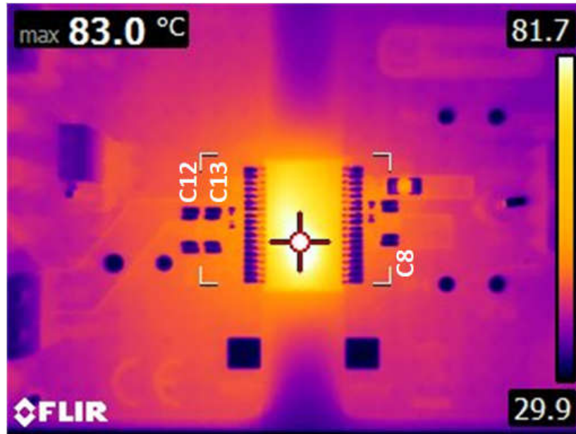
Figure 12-6. Thermal Image
