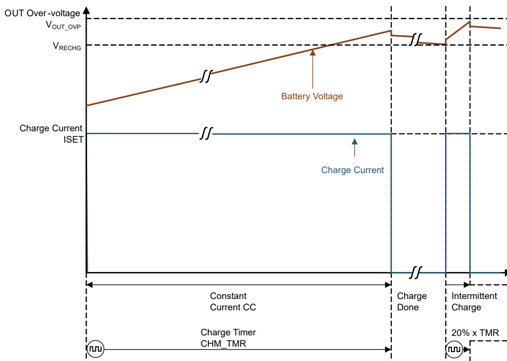
Figure 2-1. BQ25172 Charge Profile
