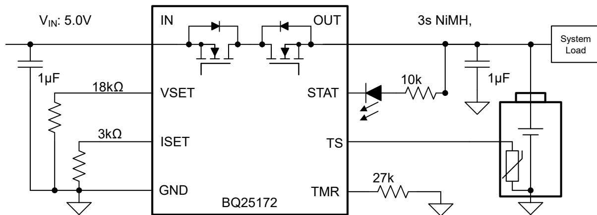
Figure 6-1. Block Diagram
