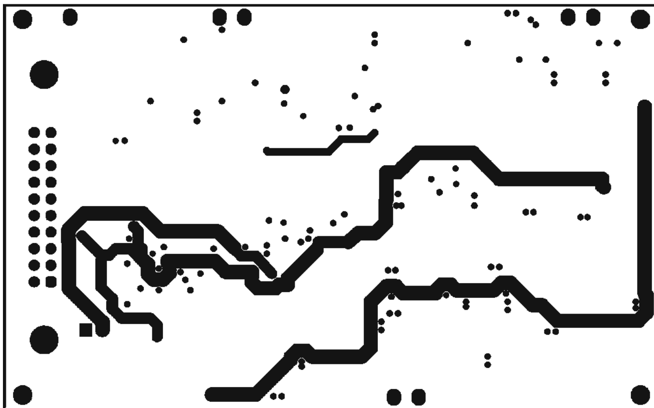
Figure 14. Signal Layer 1
