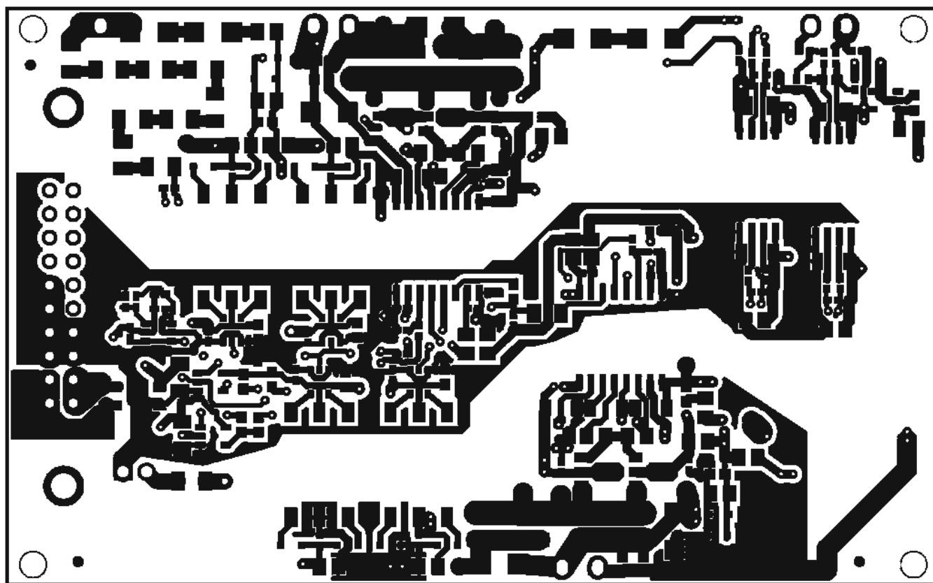
Figure 13. Top Layer
