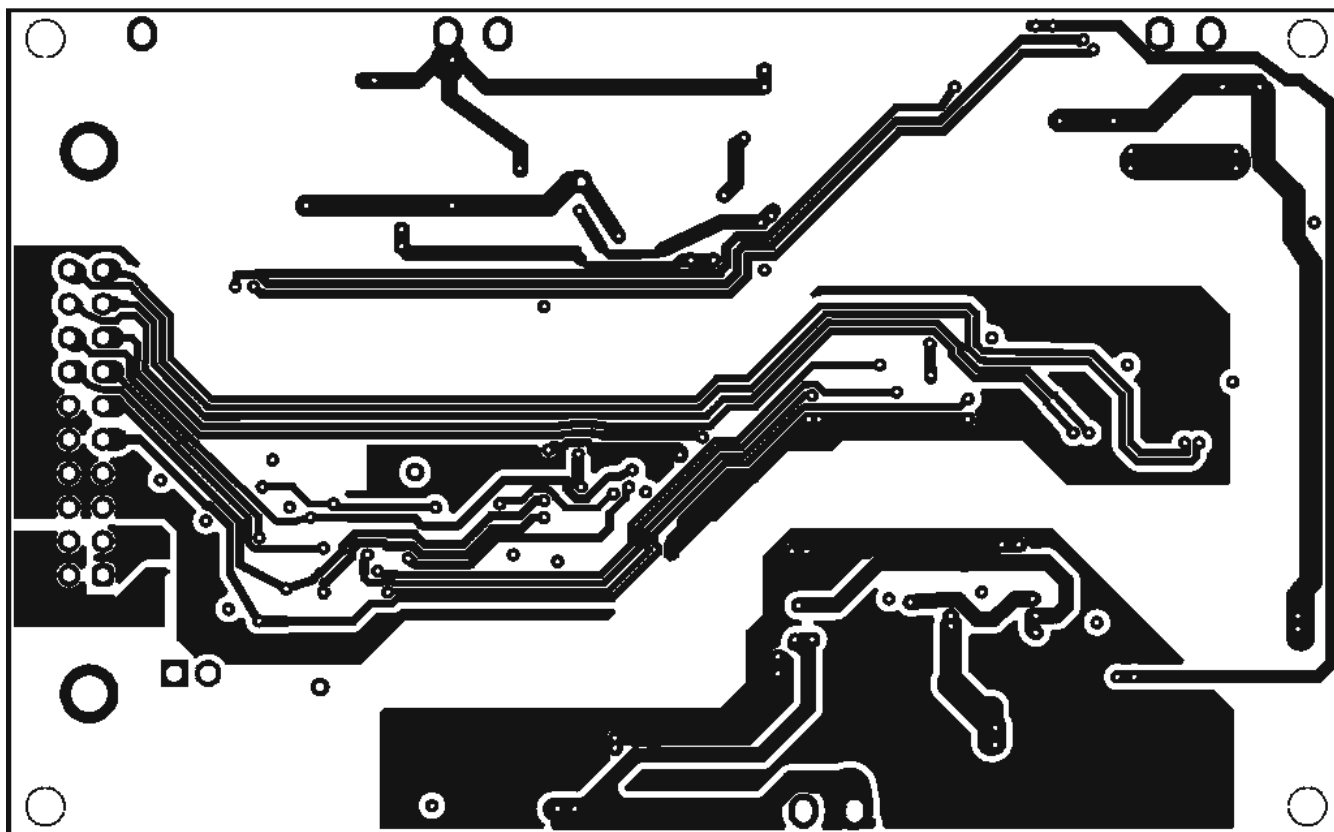
Figure 16. Bottom Layer
