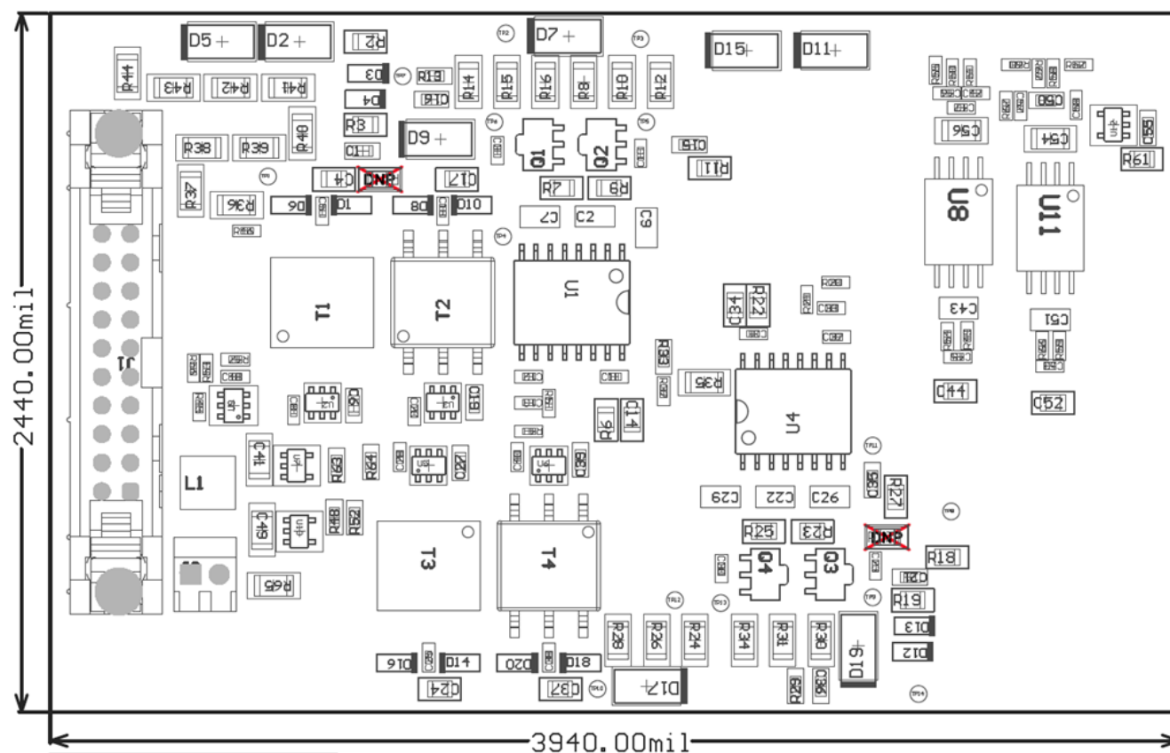
Figure 12. Component Placement
