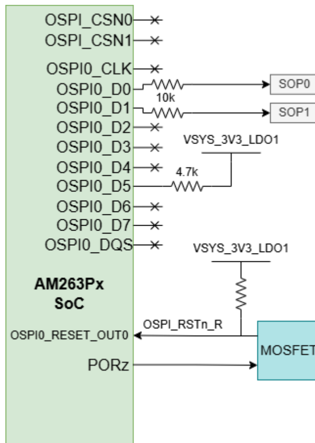
Figure 2-16. OSPI Interface
