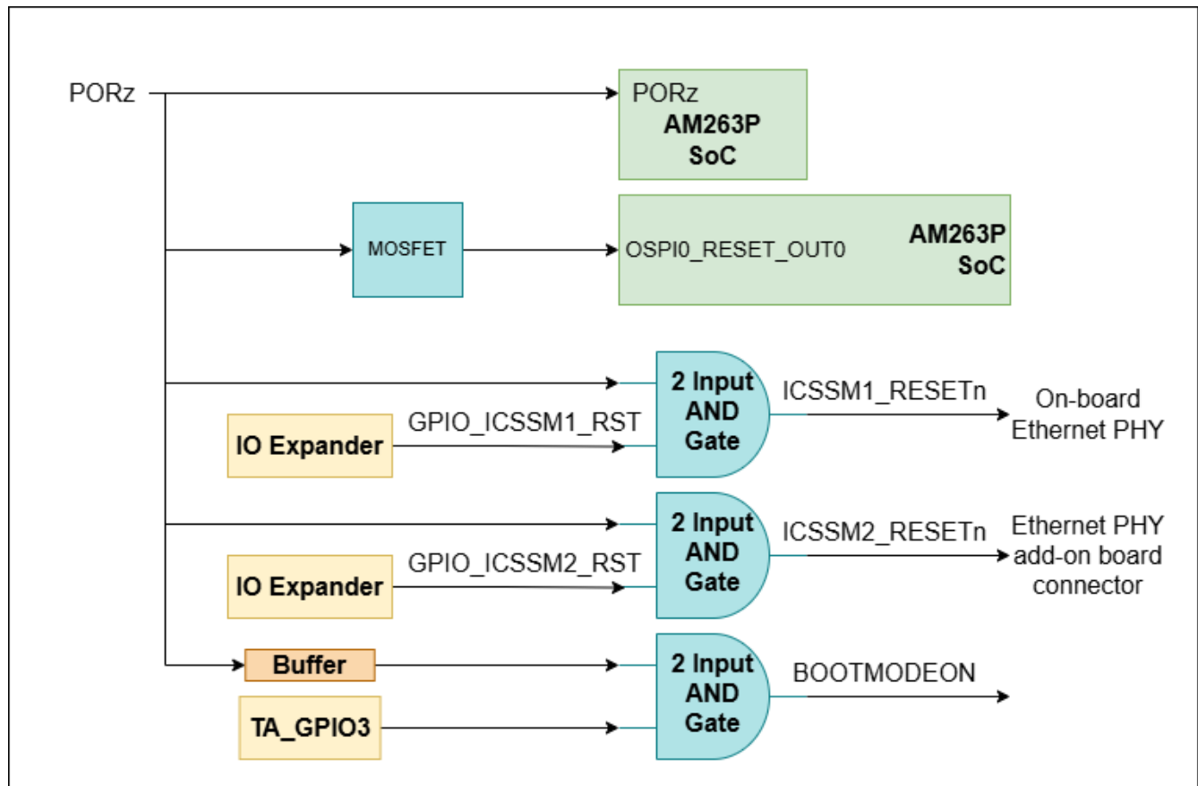
Figure 2-9. PORz Reset Signal Tree
