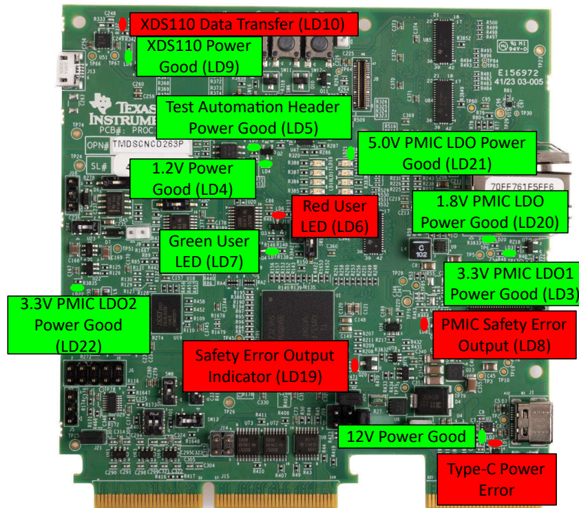
Figure 2-3. Power Status LEDs
