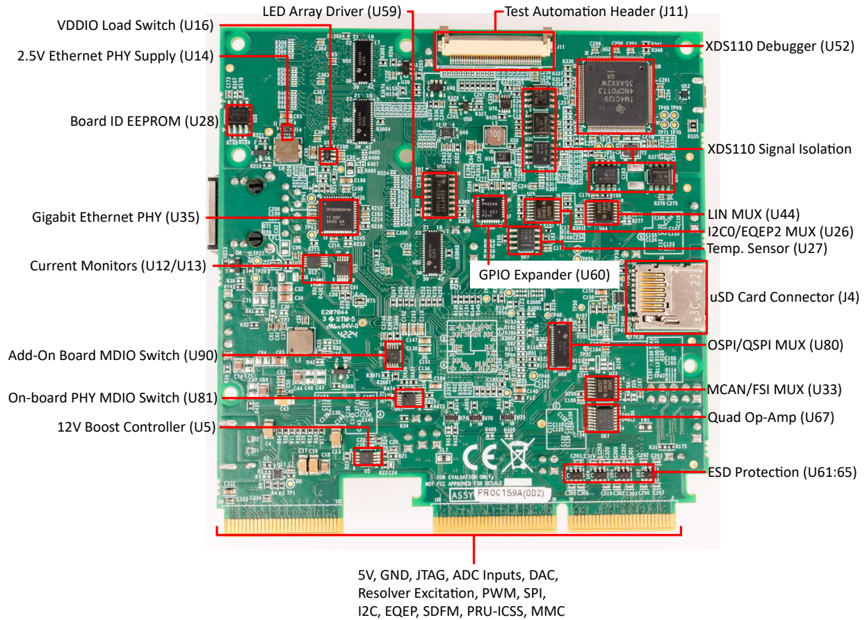
Figure 1-2. Component Identification (Back View)
