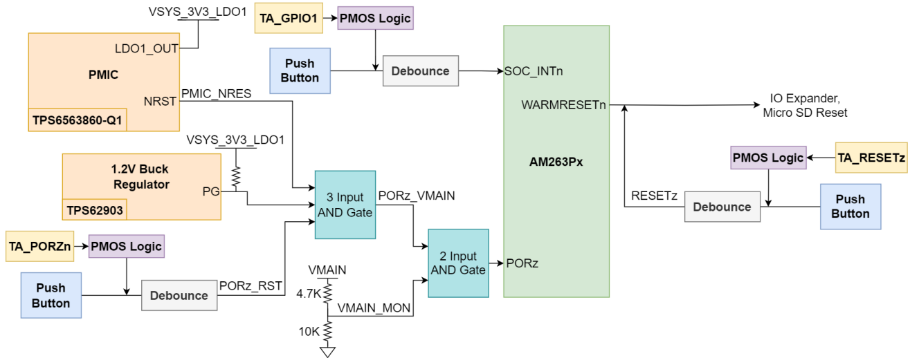
Figure 2-8. Reset Architecture
