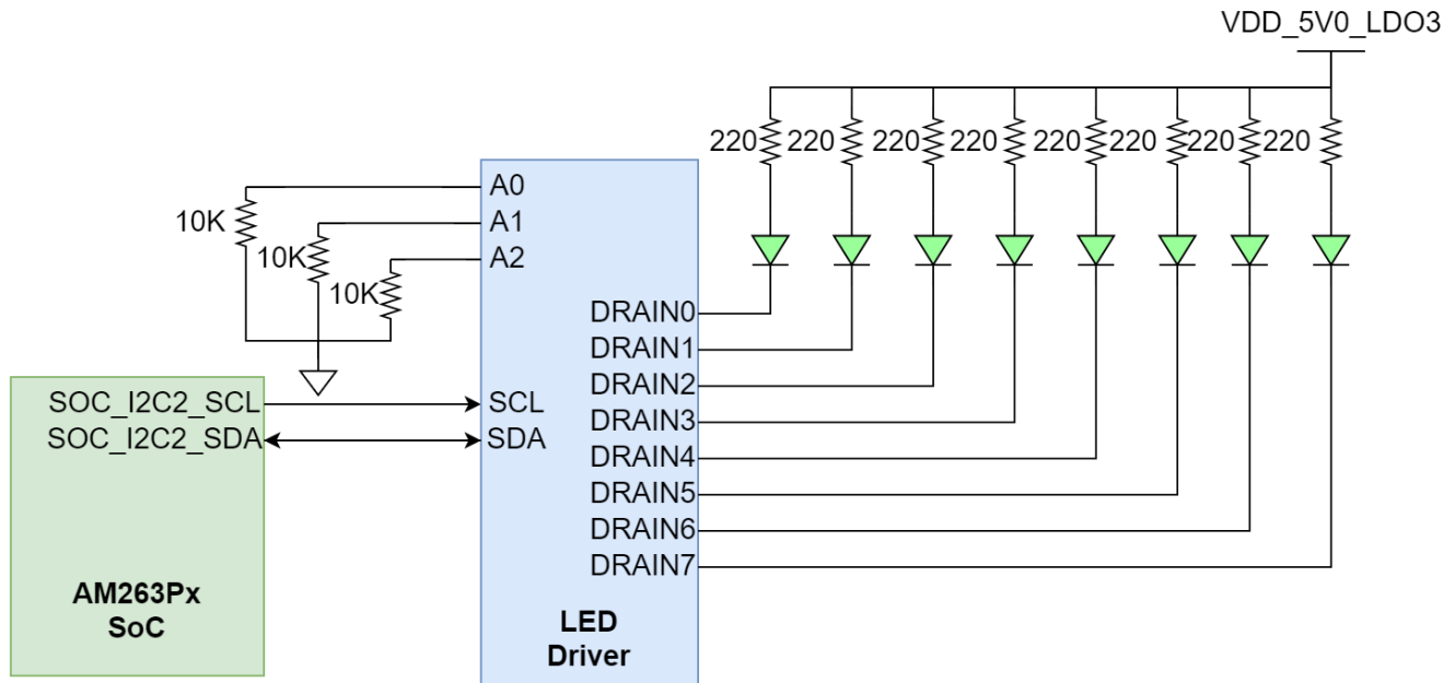
Figure 2-22. Industrial Application LED Driver
