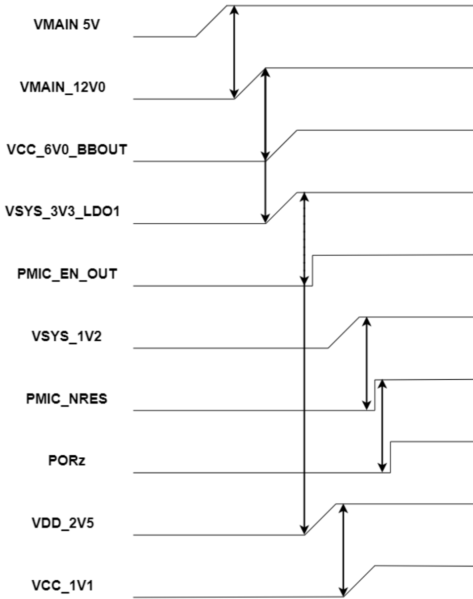
Figure 2-5. Power Sequence Diagram
