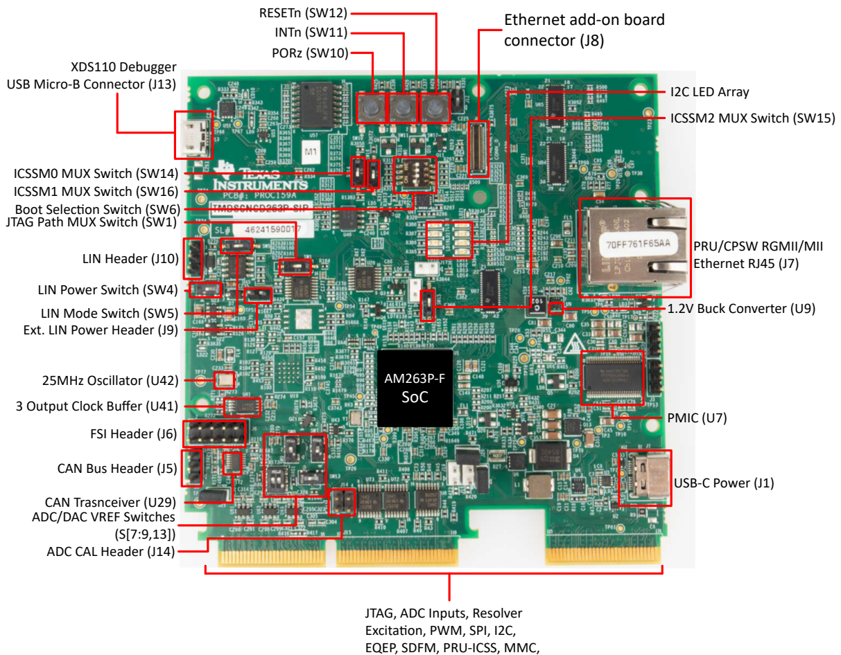
Figure 1-1. Component Identification (Front View)
