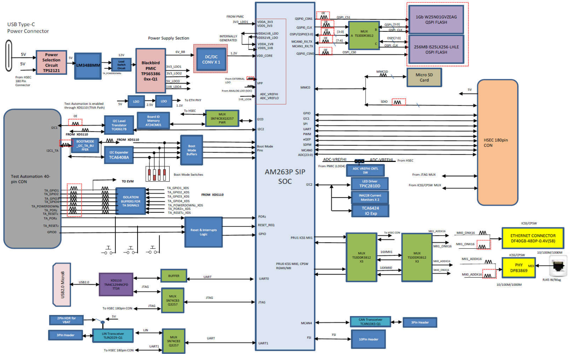
Figure 2-7. AM263Px-SIP Control Card Block Diagram
