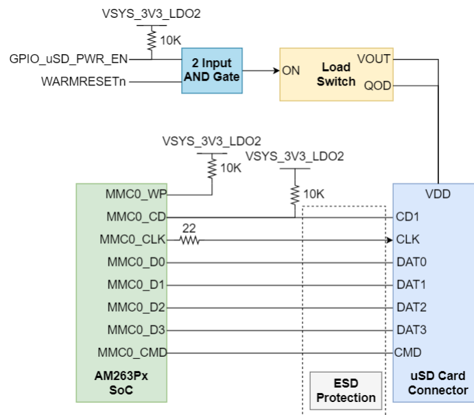
Figure 2-32. Micro-SD Connector Interface
