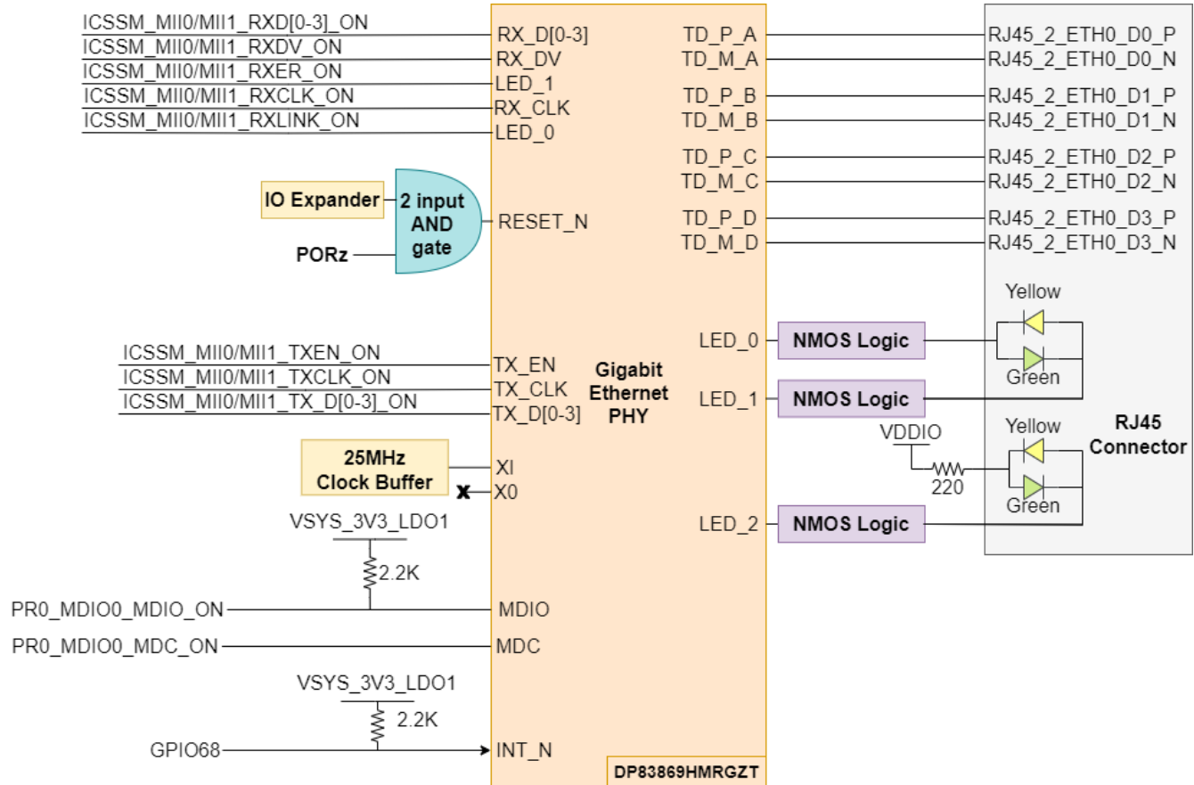
Figure 2-19. Control Card On Board Ethernet PHY
