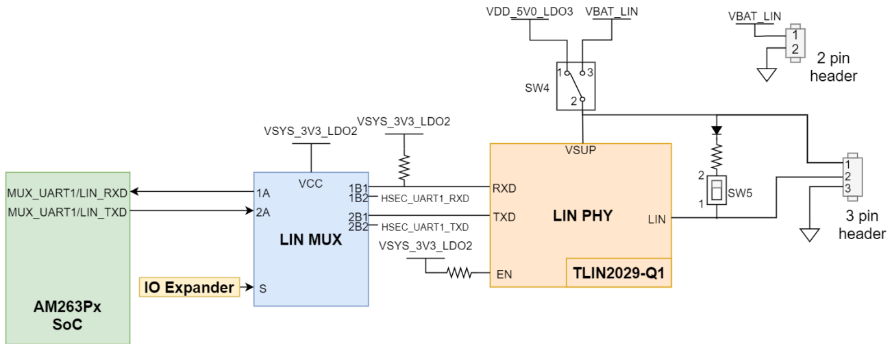
Figure 2-31. LIN PHY
