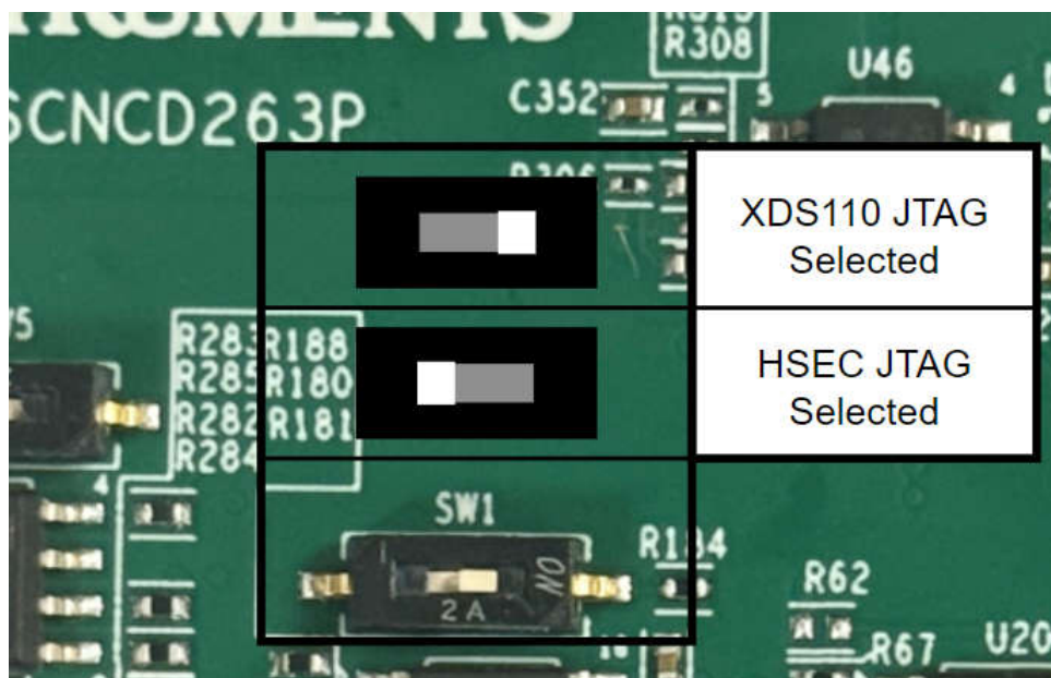
Figure 2-14. JTAG Path Switch Position
