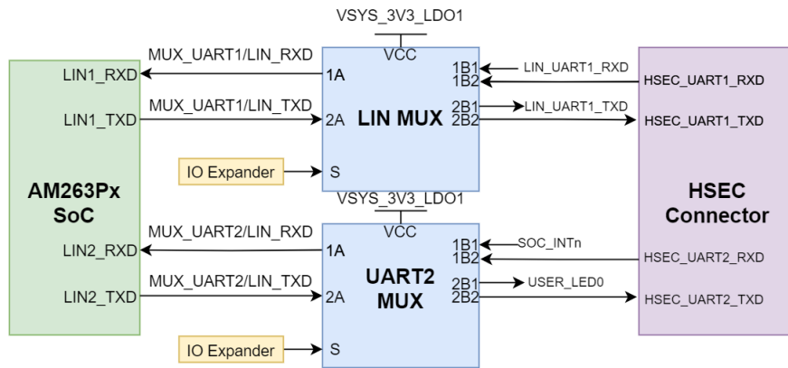
Figure 2-25. UART 1:2 MUX to HSEC
