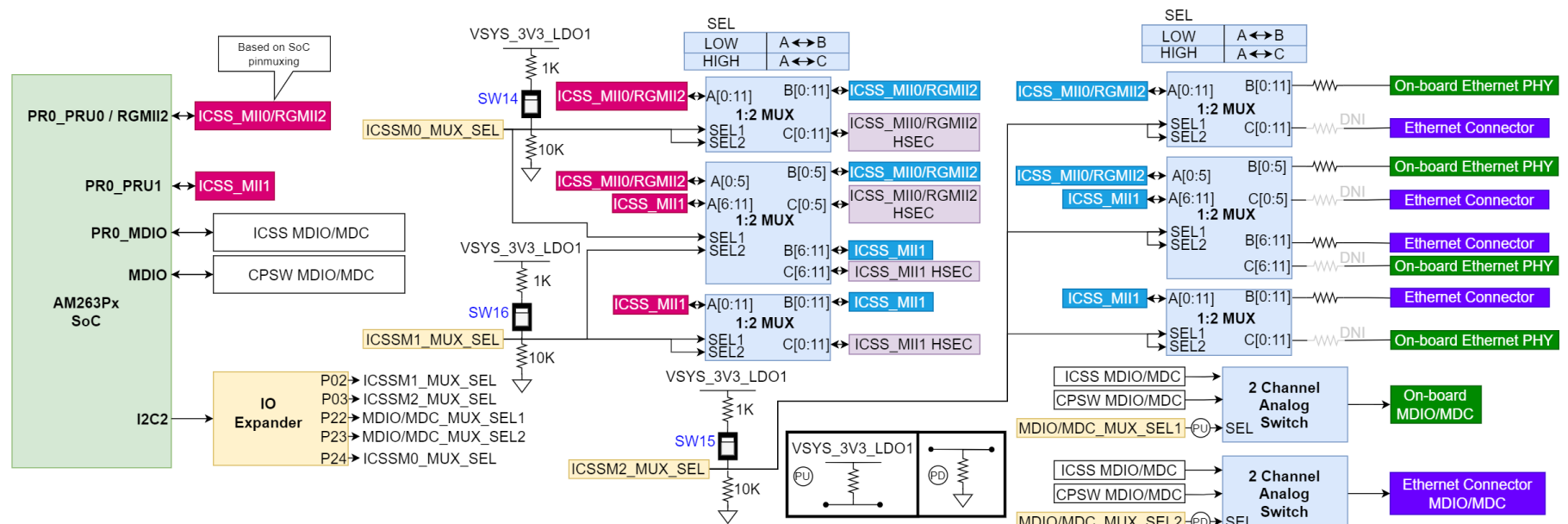
Figure 2-18. Ethernet Routing Overview
