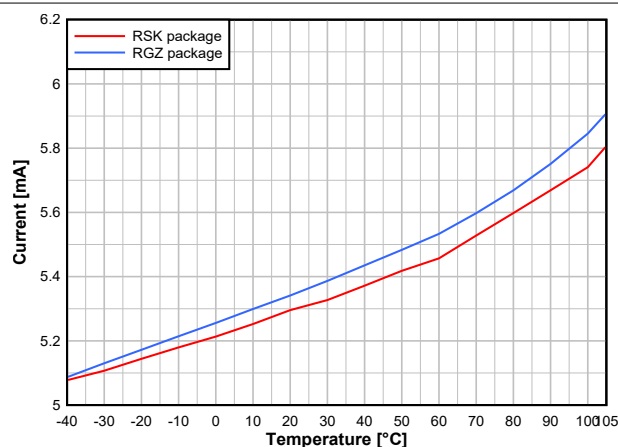
Figure 7-6. RX Current vs. Temperature (50kbps, 868.3MHz, VDD5 = 3.6V)
