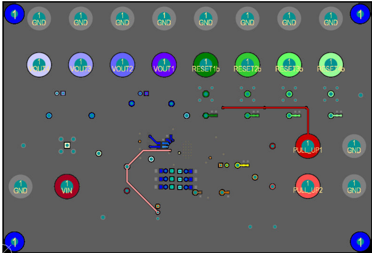
Figure 9-6. Printed Circuit Board Layout Example: Bottom Layer
