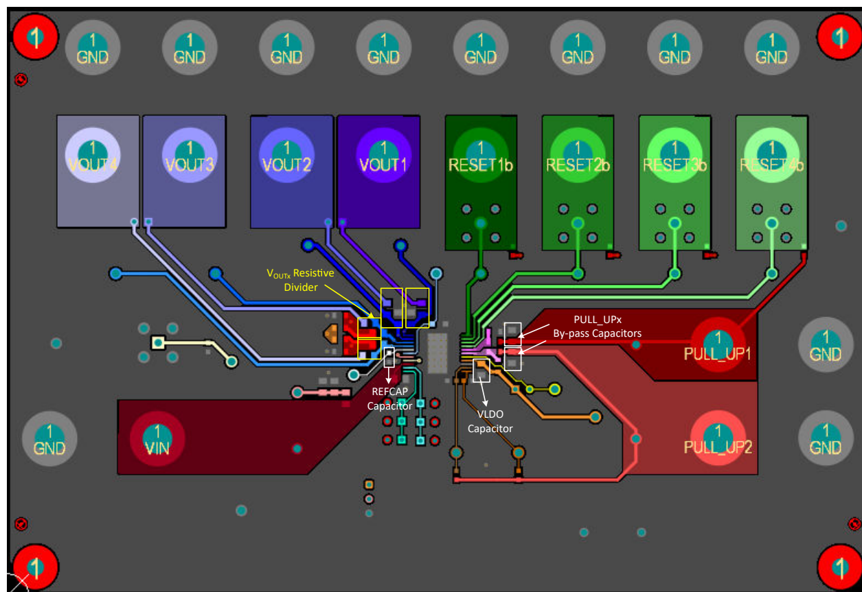
Figure 9-5. Printed Circuit Board Layout Example: Top Layer
