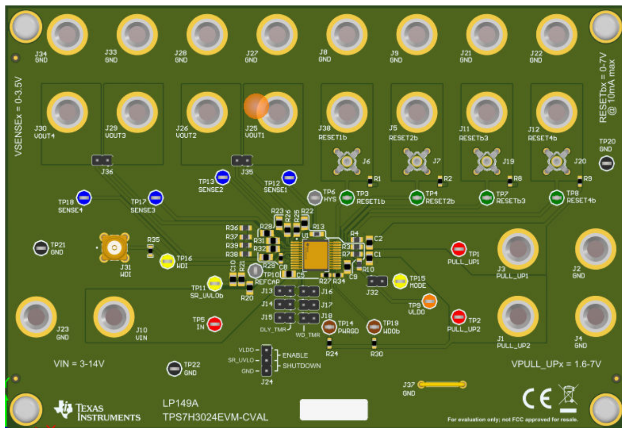
Figure 9-7. Printed Circuit Board Layout Example: Top Layer 3D View
