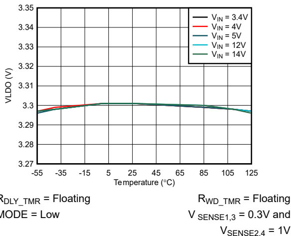
Figure 6-17. VLDO vs Temperature Across V_{IN}
