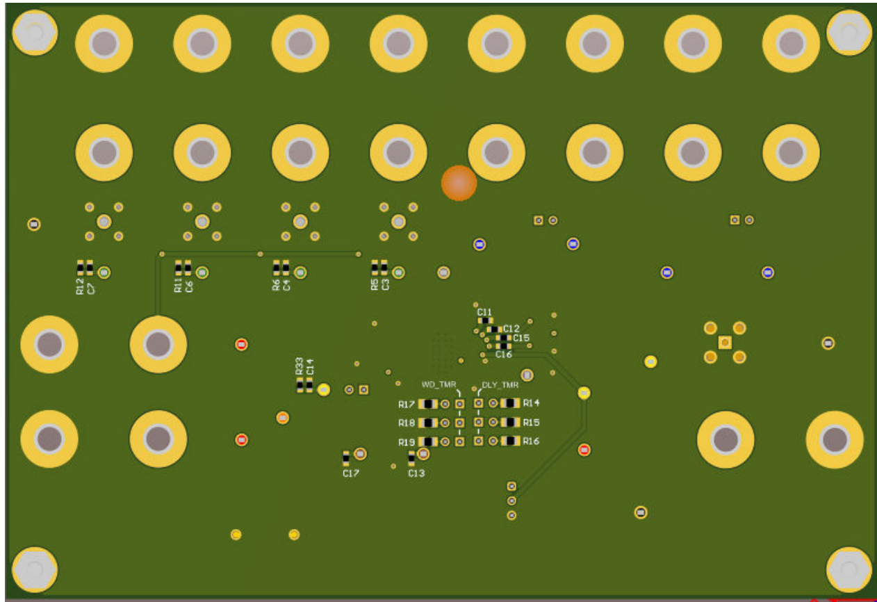
Figure 9-8. Printed Circuit Board Layout Example: Bottom Layer 3D View
