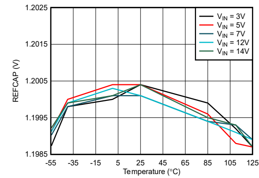
Figure 6-15. REFCAP vs Temperature Across V_{IN}
