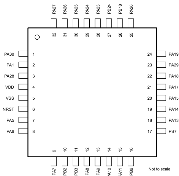
Figure 6-4. 32-pin RHB (VQFN) Package
