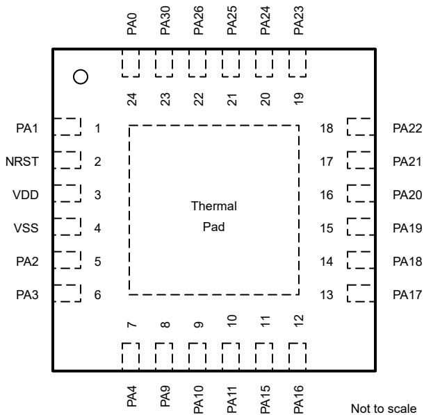
Figure 6-7. 24-pin RGE (VQFN) Package
