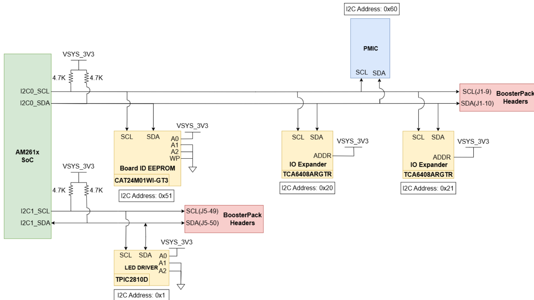
Figure 2-19. LP-AM261 I2C Interface
