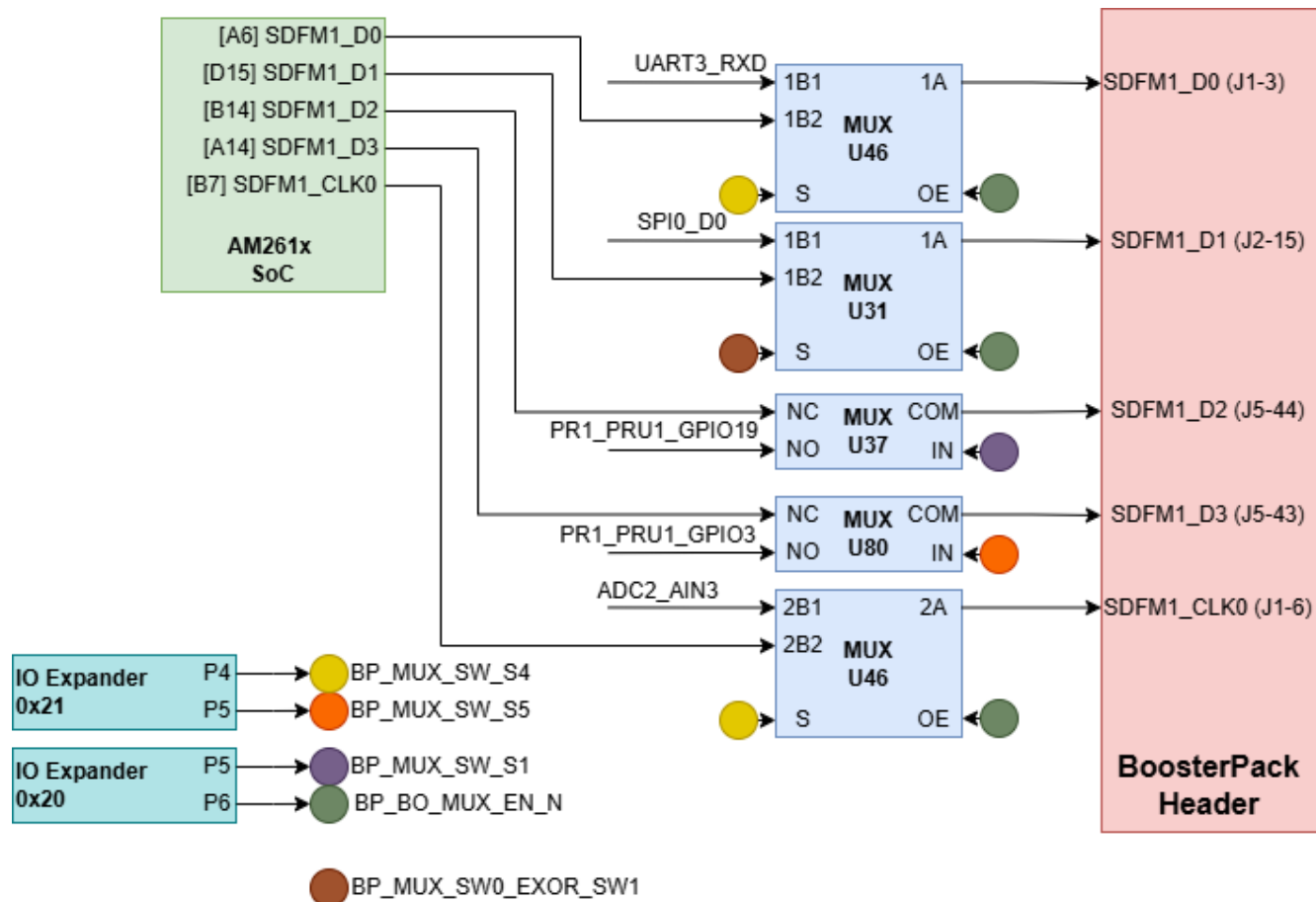
Figure 2-25. SDFM1
