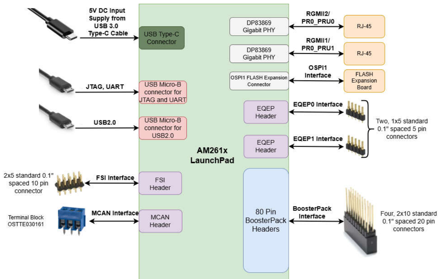
Figure 1-1. System Architecture
