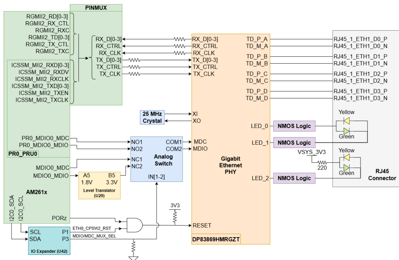
Figure 2-17. Ethernet PHY 0
