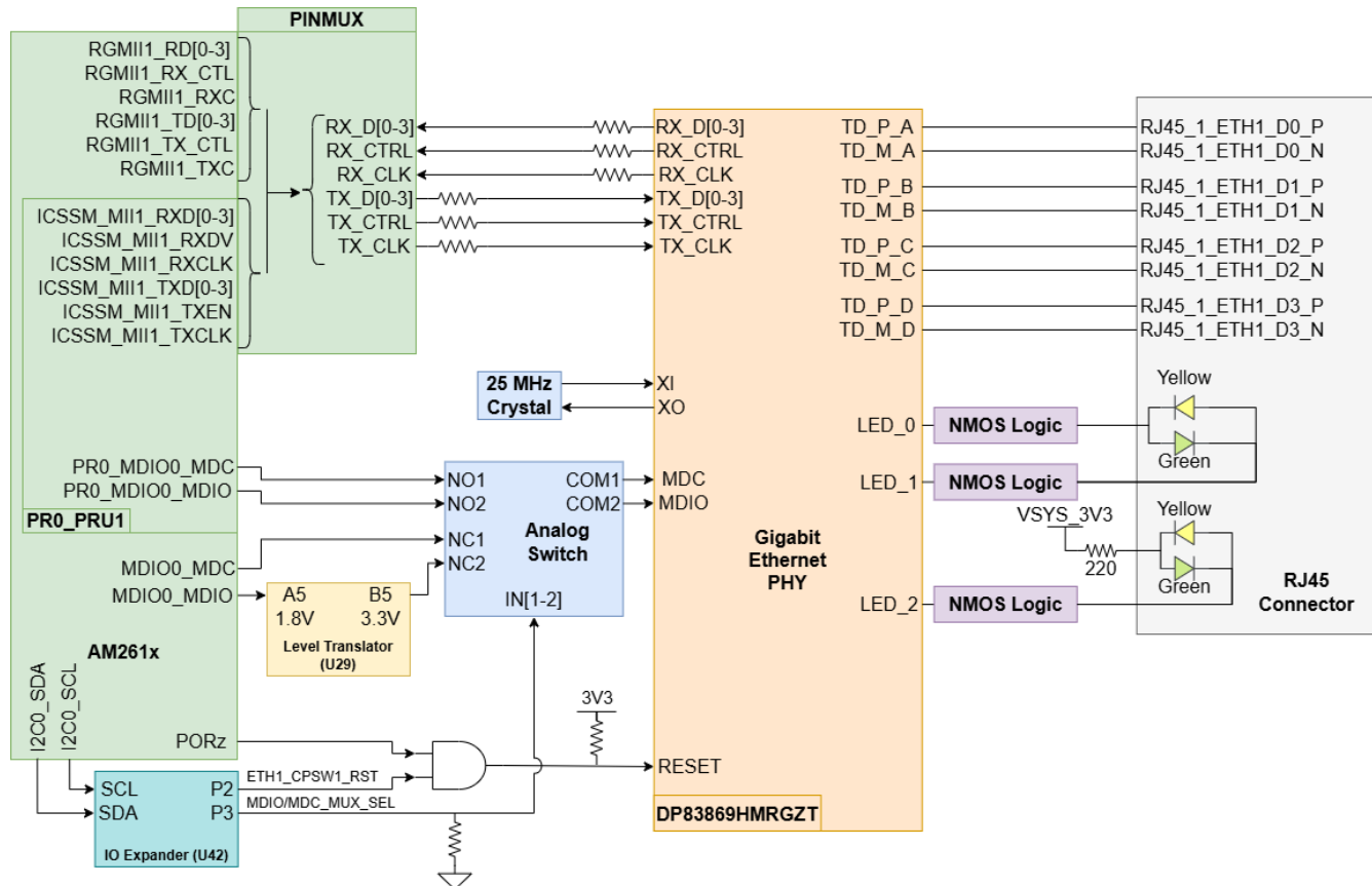
Figure 2-18. Ethernet PHY 1
