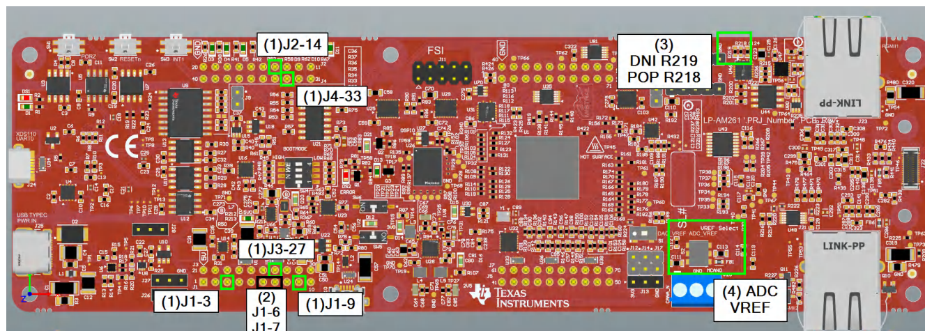
Figure 6-2. LP-AM261 Modifications for BP-AMC0106-LMG-MD Demo
