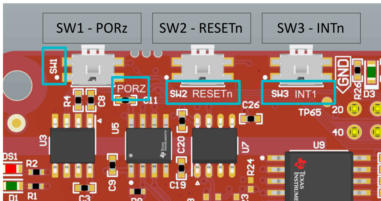
Figure 2-6. Push Buttons
