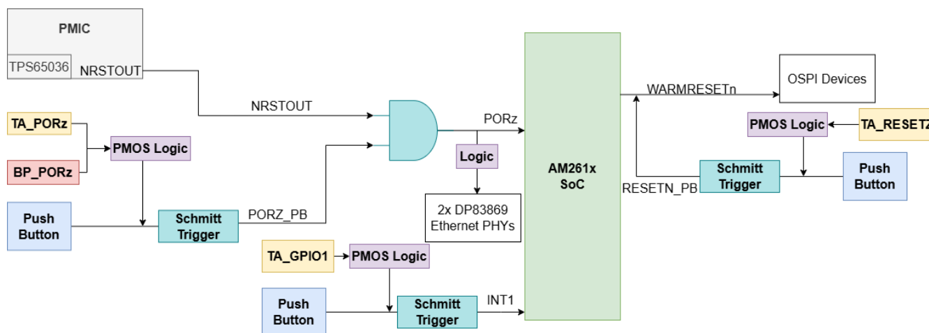
Figure 2-7. Reset Architecture
