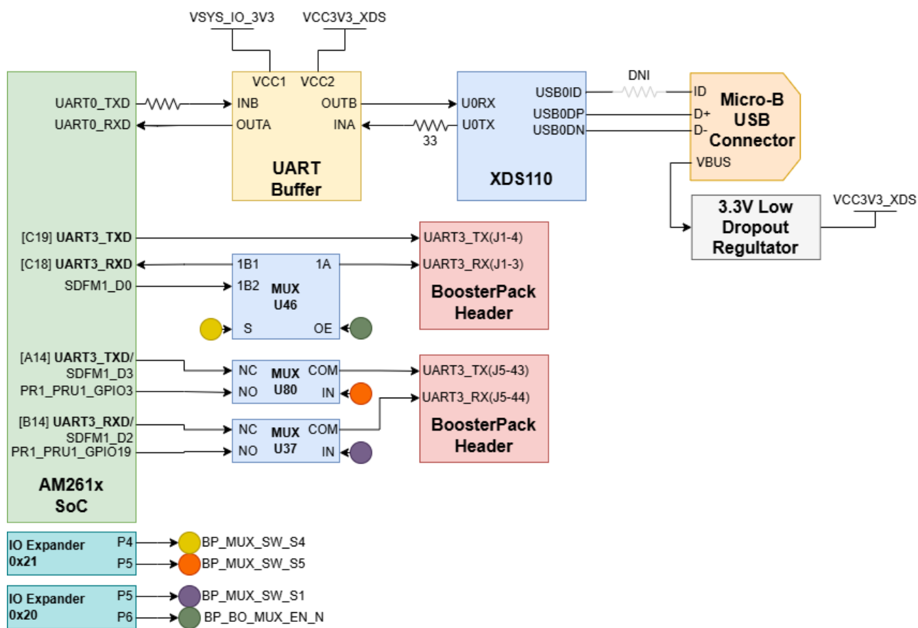
Figure 2-22. LP-AM261 UART Interface
