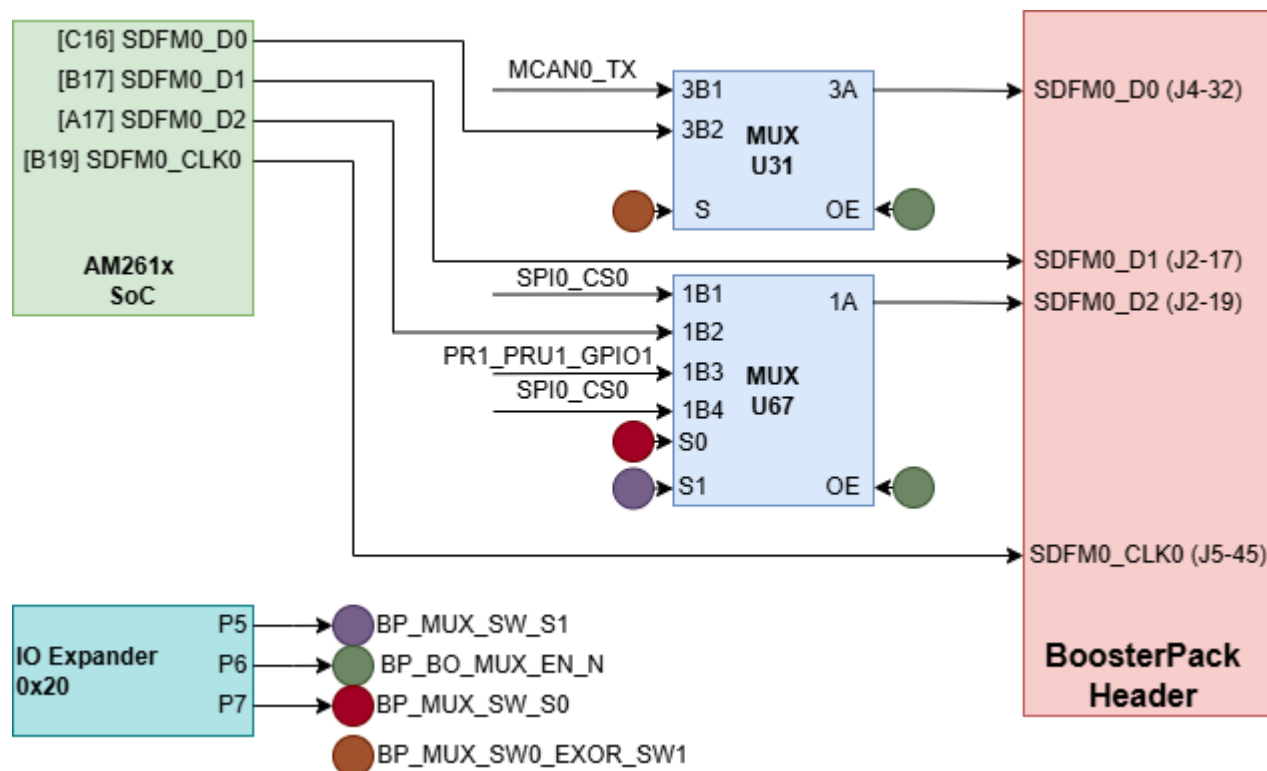
Figure 2-24. SDFM0
