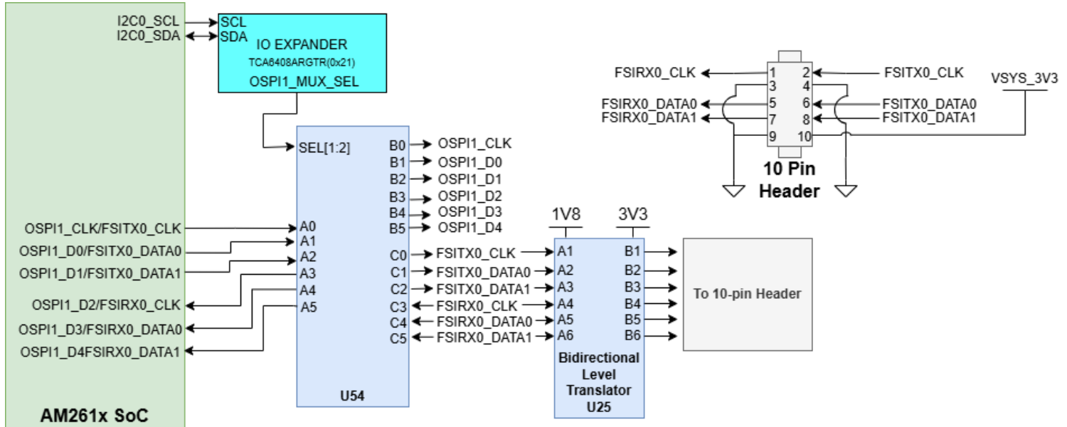
Figure 2-26. LP-AM261 FSI Interface
