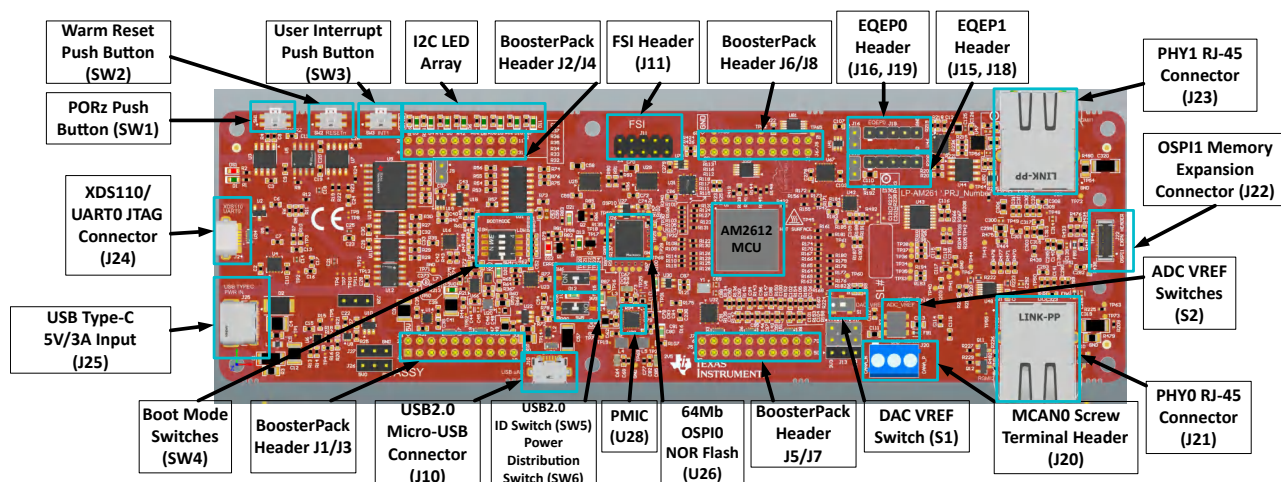
Figure 1-2. AM261x LaunchPad Top Components Identification
