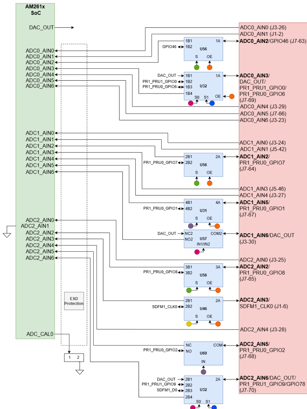
Figure 2-30. ADC/DAC Interface
