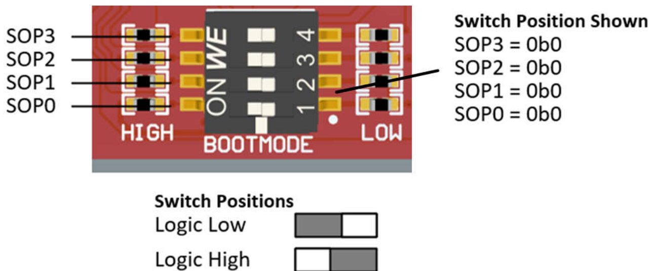
Figure 2-11. Boot mode DIP Switch Positions - LP AM261x E2 SW1 SOP Switches
