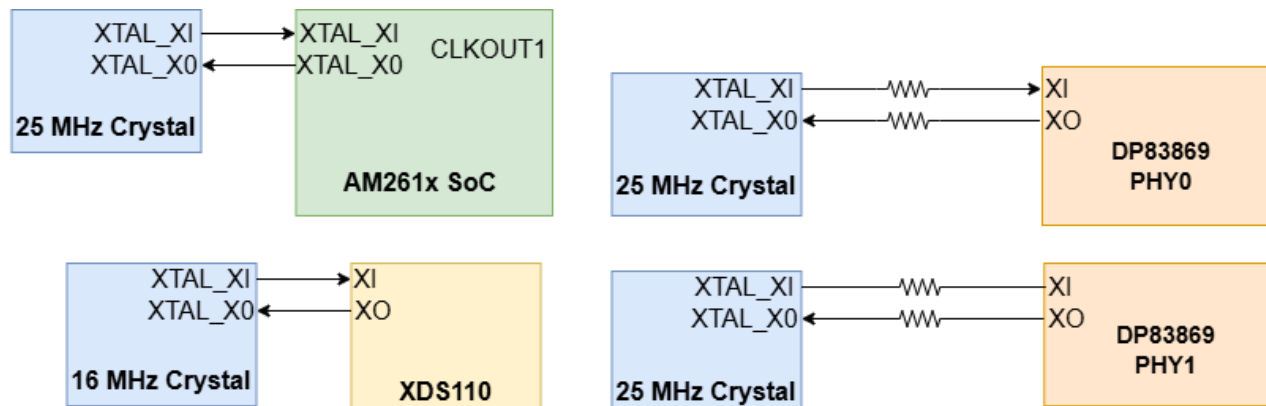
Figure 2-10. AM261x LaunchPad Clock Tree
