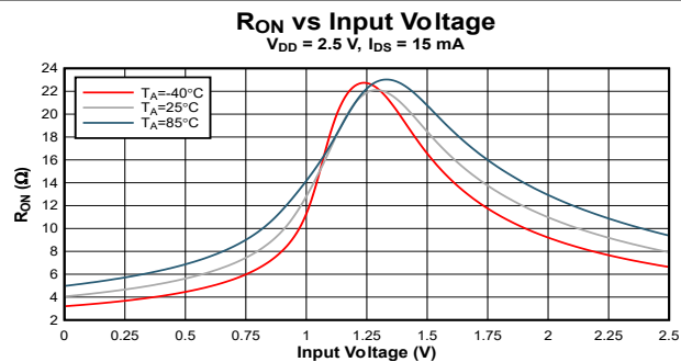
Figure 5-1. R ON vs Input Voltage, V DD = 2.5V, I DS = 15mA
