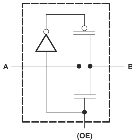
Simplified Schematic, Each FET Switch
