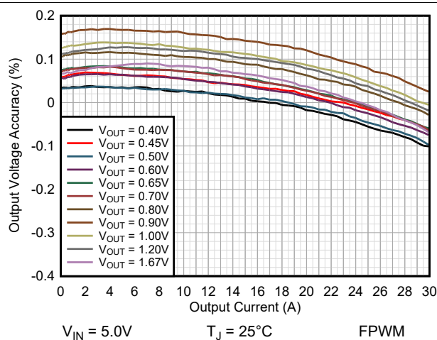
Figure 9-18. Load Regulation TPSM8287B30xx
