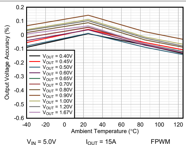
Figure 9-19. Vout Accuracy vs Temperature TPSM8287B30xx
