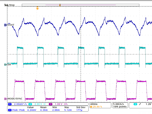
Figure 9-23. PWM-DCM Operation TPSM8287B30HAPx
