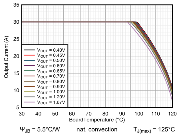
Figure 9-35. Safe Operating Area TPSM8287B30xx V_{IN} = 5.0\text{V}
