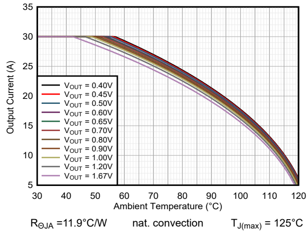
Figure 9-32. Safe Operating Area TPSM8287B30xx V_{IN} = 3.3\text{V}
