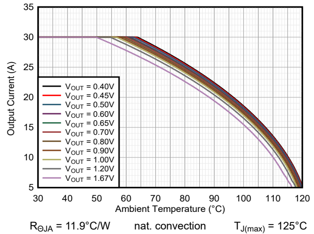
Figure 9-33. Safe Operating Area TPSM8287B30xx V_{IN} = 5.0\text{V}
