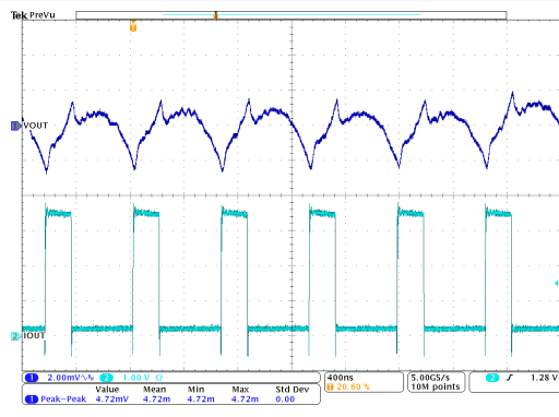
Figure 9-20. Load Transient TPSM8287B30HAPx
