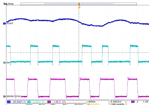
Figure 9-27. Synchronization to a Random External Clock TPSM8287B30HAPx
