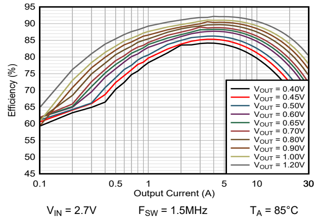
Figure 9-9. Efficiency TPSM8287B30xx PSM
