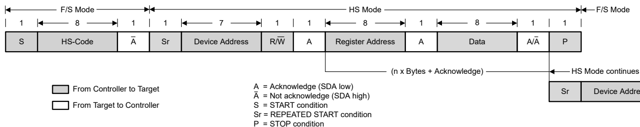
Figure 7-24. Data Transfer Format in HS-Mode
