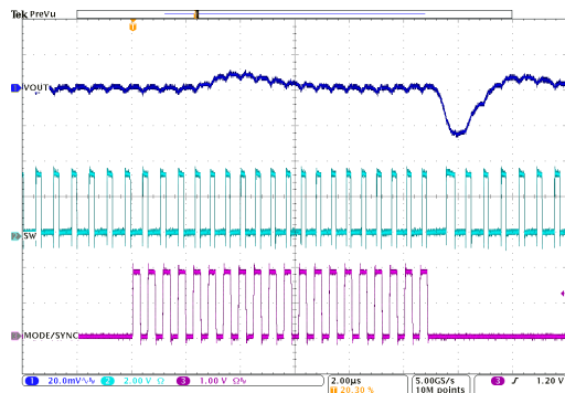
Figure 9-26. Adding and Removing an External Clock TPSM8287B30HAPx
