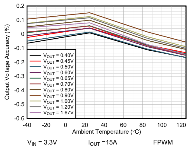
Figure 9-17. Vout Accuracy vs Temperature TPSM8287B30xx
