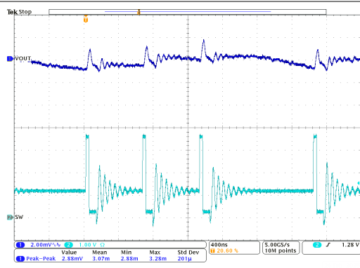
Figure 9-22. PWM-CCM Operation TPSM8287B30HAPx
