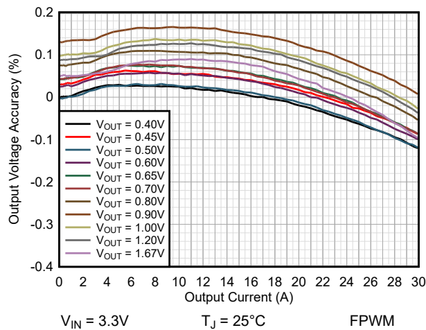
Figure 9-16. Load Regulation TPSM8287B30xx
