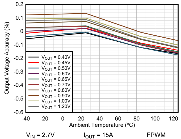
Figure 9-15. Vout Accuracy vs Temperature TPSM8287B30xx
