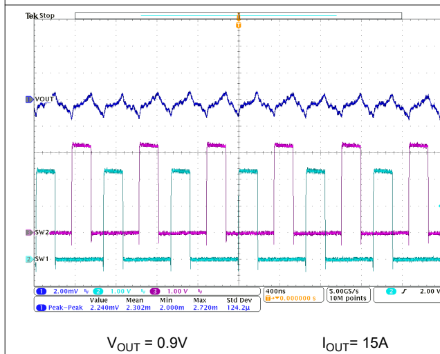
Figure 9-45. PWM-CCM Operation TPSM8287B30HAPx
