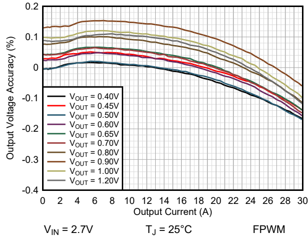
Figure 9-14. Load Regulation TPSM8287B30xx
