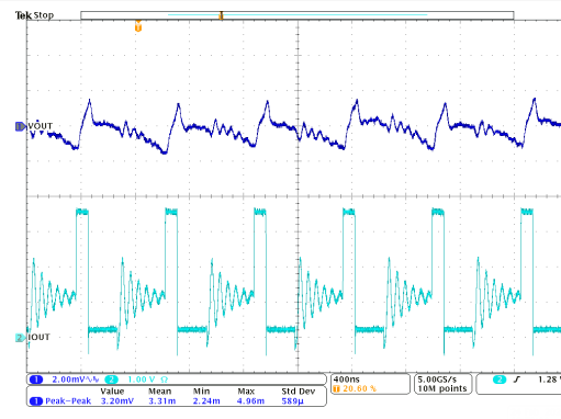
Figure 9-21. Load Transient TPSM8287B30HAPx
