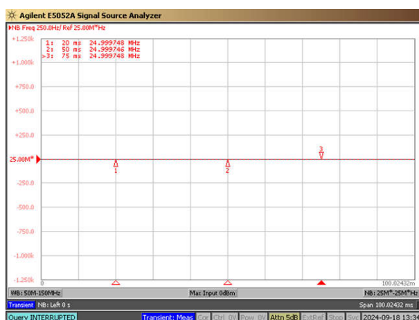
Figure 8-11. During 1500g Mechanical Shock at 25MHz and 25°C, Z-Axis
