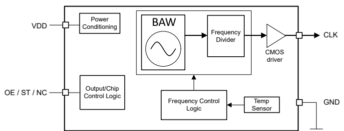
CDC6Cx-Q1 Simplified Block Diagram
