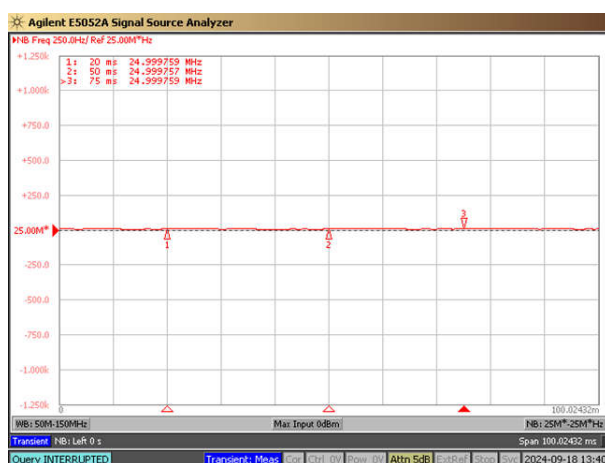
Figure 8-9. During 1500g Mechanical Shock at 25MHz and 25°C, Y-Axis
